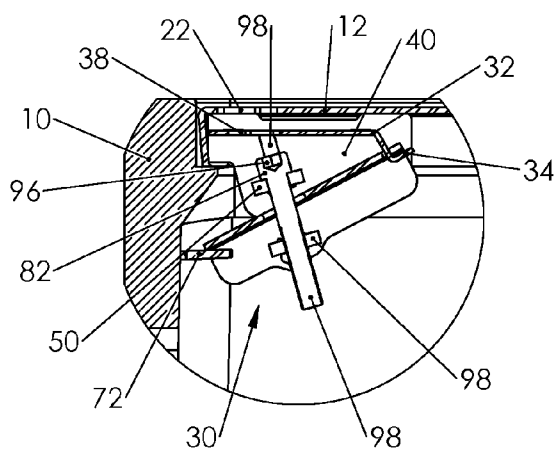
DETAIL 1C OF FIG. 1B
