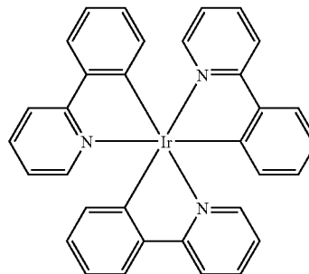
\text{Ir(ppy)}_3
