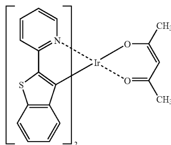
\text{Btp}_2\text{Ir(acac)}
