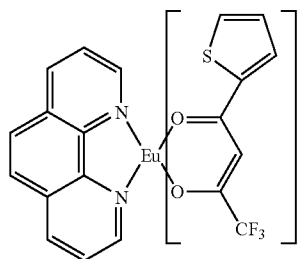
\text{Eu(TTA)}_3\text{phen}
