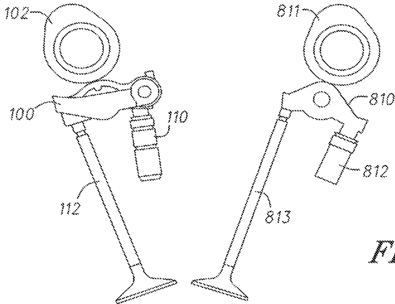
DVVL INTAKE VALVE LINE
