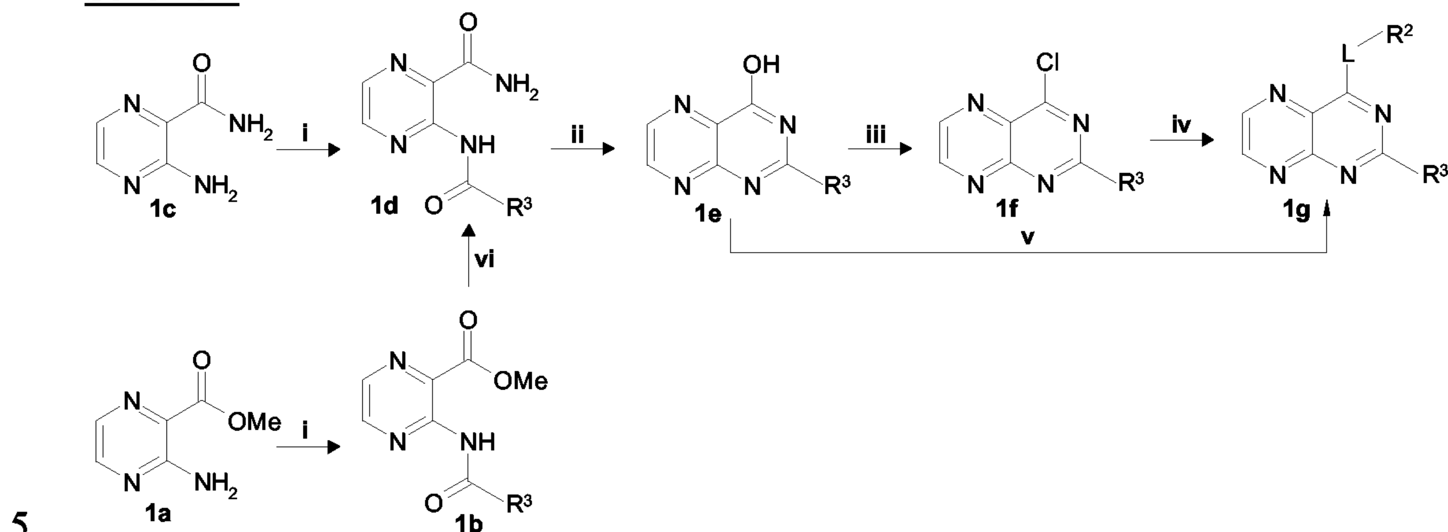
Scheme 1
