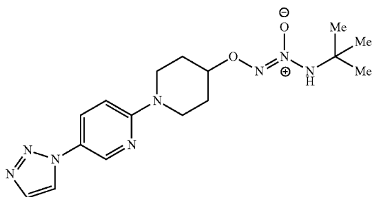
O 2 -{1-[5-(1H-1,2,3-triazol-1-yl)pyridin-2-yl]piperidin-4-yl}1-(N-tert-butylamino)diazen-1-ium-1,2-diolate
