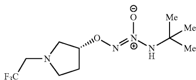
O 2 -[(3R)-1-(2,2,2-trifluoroethyl)pyrrolidin-3-yl]1-(N-tert-butylamino) diazen-1-ium-1,2-diolate
