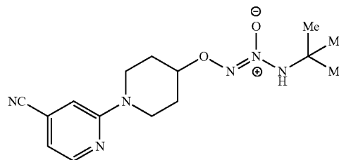
O 2 -[1-(4-cyanopyridin-2-yl)piperidin-4-yl]1-(N-tert-butylamino)diazen-1-ium-1,2-diolate
