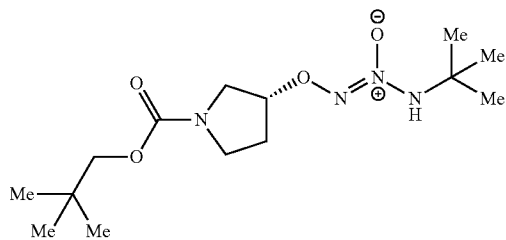
O 2 -{(3R)-1-[(2,2-dimethylpropoxy)carbonyl]pyrrolidin-3-yl}1-(N-tert-butylamino)diazen-1-ium-1,2-diolate
