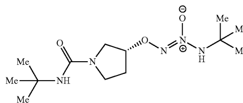
O 2 -[(3R)-1-(tert-butylcarbonyl)pyrrolidin-3-yl]1-(N-tert-butylamino) diazen-1-ium-1,2-diolate
