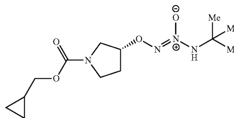
O 2 -{(3R)-1-[(cyclopropylmethoxy)carbonyl]pyrrolidin-3-yl}1-(N-tert-butylamino)diazen-1-ium-1,2-diolate
