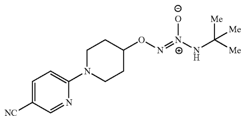
O 2 -[1-(5-cyanopyridin-2-yl)piperidin-4-yl]1-(N-tert-butylamino)diazen-1-ium-1,2-diolate
