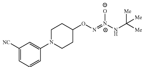
O 2 -[1-(3-cyanophenyl)piperidin-4-yl]1-(N-tert-butylamino)diazen-1-ium-1,2-diolate
