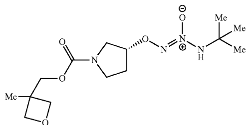
O 2 -[(3R)-1-[(3-methyloxetan-3-yl)methoxy]carbonyl]pyrrolidin-3-yl]1-(N-tert-butylamino) diazen-1-ium-1,2-diolate
