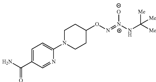
O 2 -[1-(5-carbamoylpyridin-2-yl)piperidin-4-yl]1-(N-tert-butylamino)diazen-1-ium-1,2-diolate
