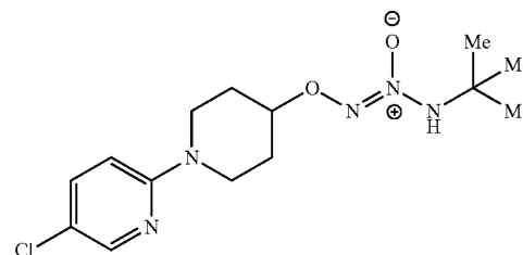
O 2 -[1-(5-chloropyridin-2-yl)piperidin-4-yl]1-(N-tert-butylamino)diazen-1-ium-1,2-diolate
