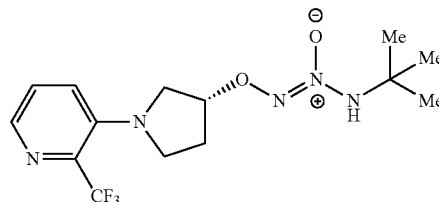
O 2 -[(3R)-1-[2-(trifluoromethyl)pyridin-3-yl]pyrrolidin-3-yl]1-(N-tert-butylamino)diazen-1-ium-1,2-diolate
