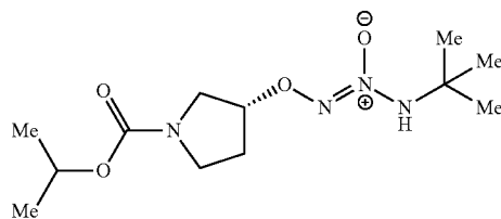
O 2 -{(3R)-1-[(propan-2-yloxy)carbonyl]pyrrolidin-3-yl}1-(N-tert-butylamino)diazen-1-ium-1,2-diolate
