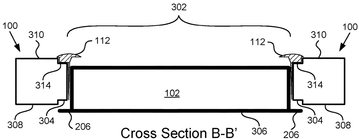
Partial Cross Section B-B' FIG. 2C
