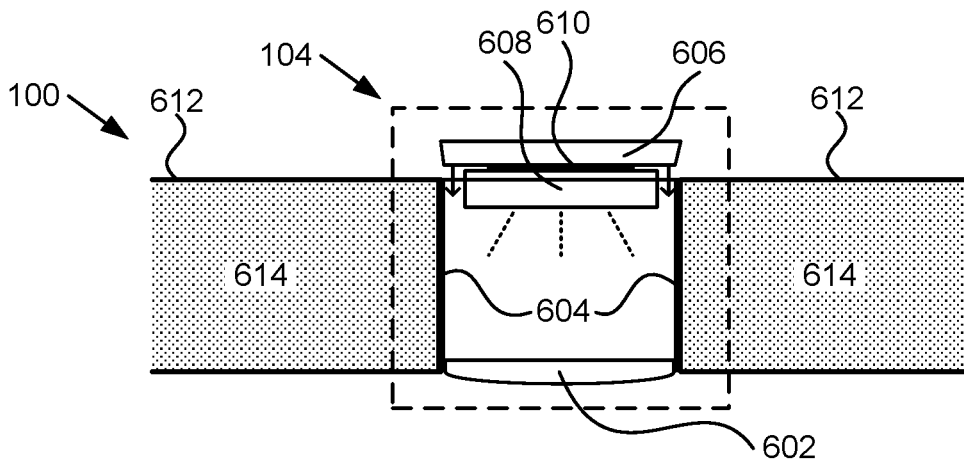
Partial Cross Section A-A'
