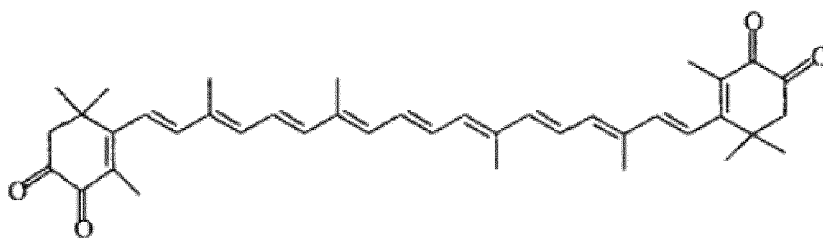
Astacene ( C_{40}H_{48}O_4 )
