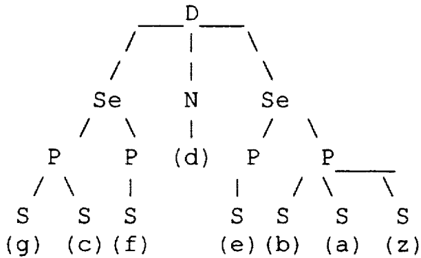
Figure 6B: Modified Document Tree (T2)
