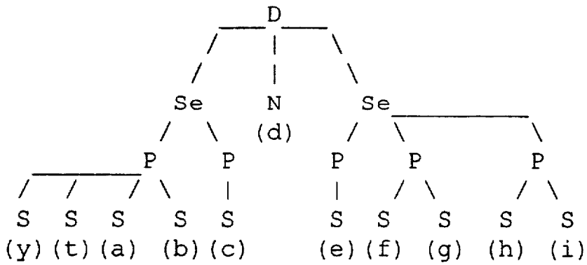
Figure 6A: Sample Document Tree (T1)
