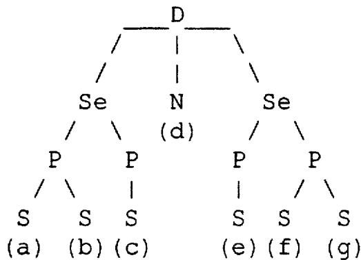
Figure 6C: Document Tree (T1') after deletion phase
