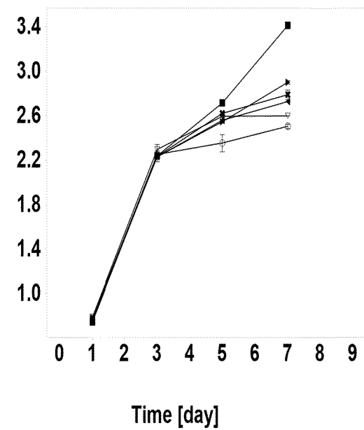
(O) Lactate Conc. [g/L]
