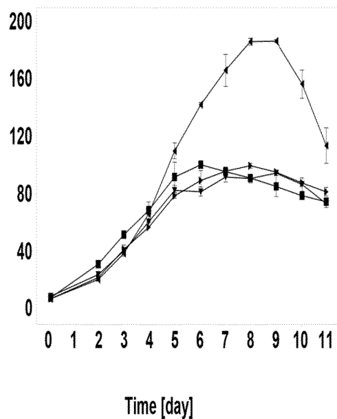
(C) Product Conc. [mg/L]
