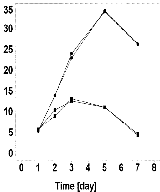
(E) Viable Cell Conc. [ 10^5 c/mL]
