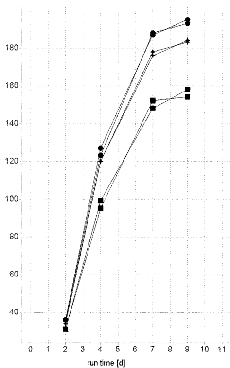
(C) Product Conc. [mg/L]
