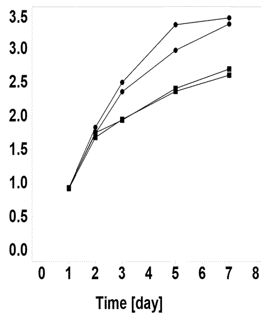
(H) Lactate Conc. [g/L]
