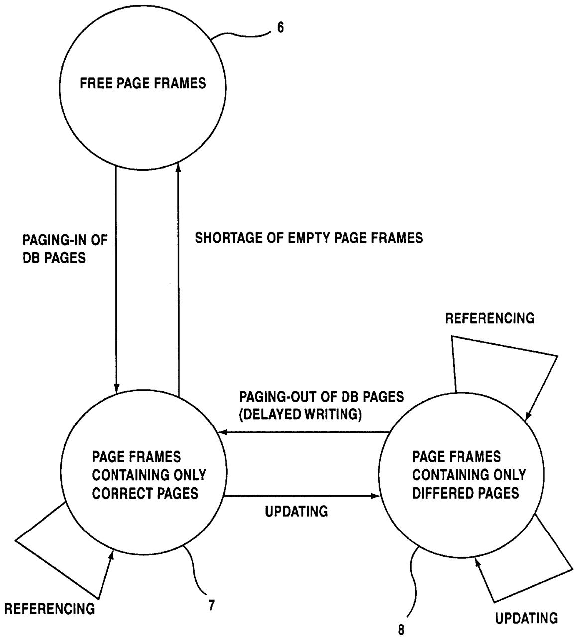
PAGE FRAME STATE TRANSITION DIAGRAM
