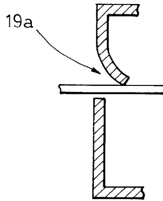
AFTER CONNECTION
