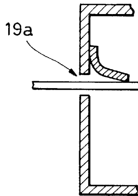
AFTER CONNECTION
