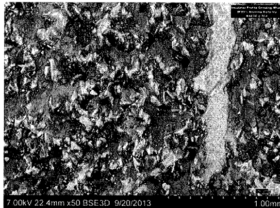
Surface of loaded grinding wheel
