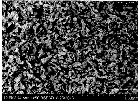
Surface of virgin wheel
