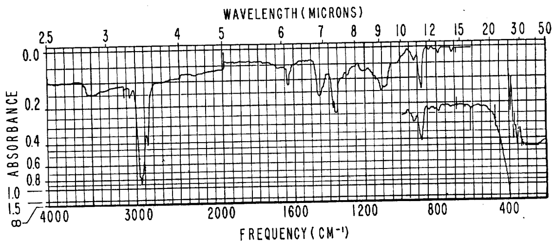
I R SPECTRUM FOR EXAMPLE XXX
