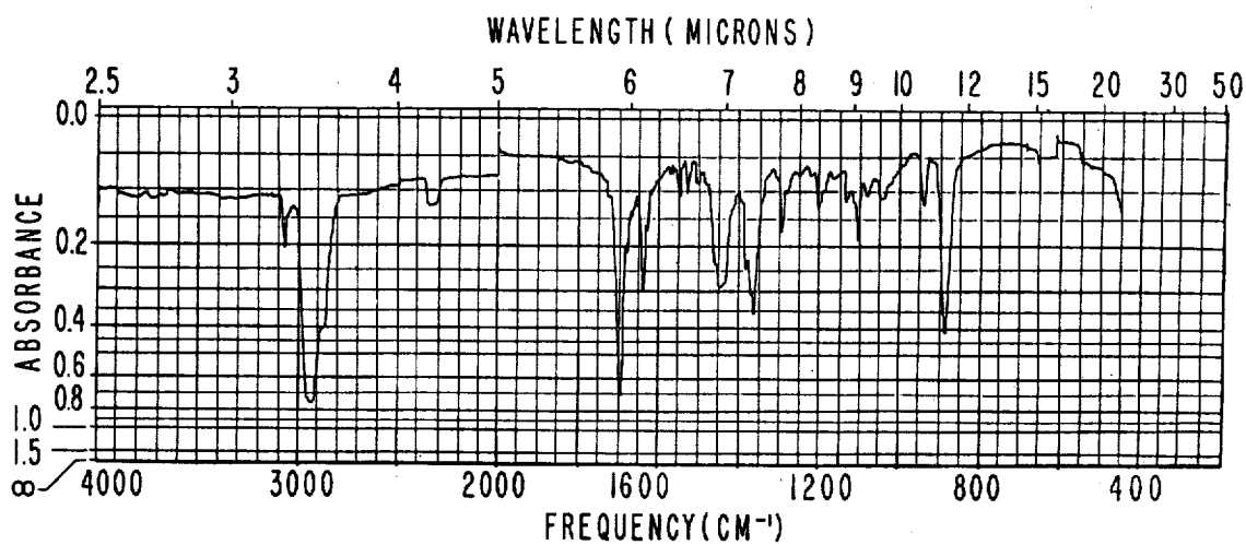
I R SPECTRUM FOR EXAMPLE XXXI
