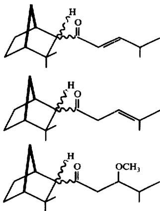
FIG. 17 illustrates the Infrared spectrum of fraction 12 of Example XX which is a mixture of the three compounds having the structures:
