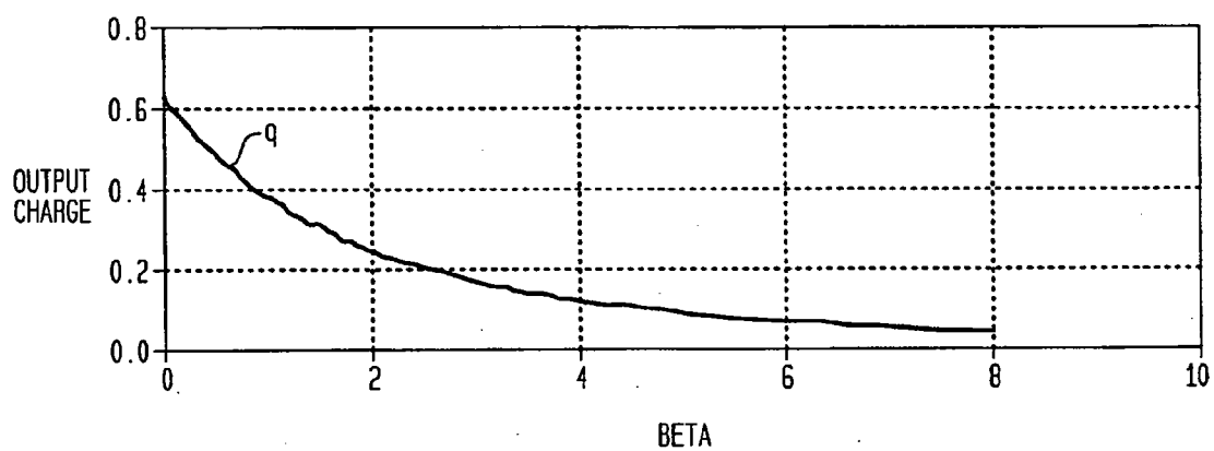
FIG. 174 UFT OUTPUT CHARGE TRANSFER
