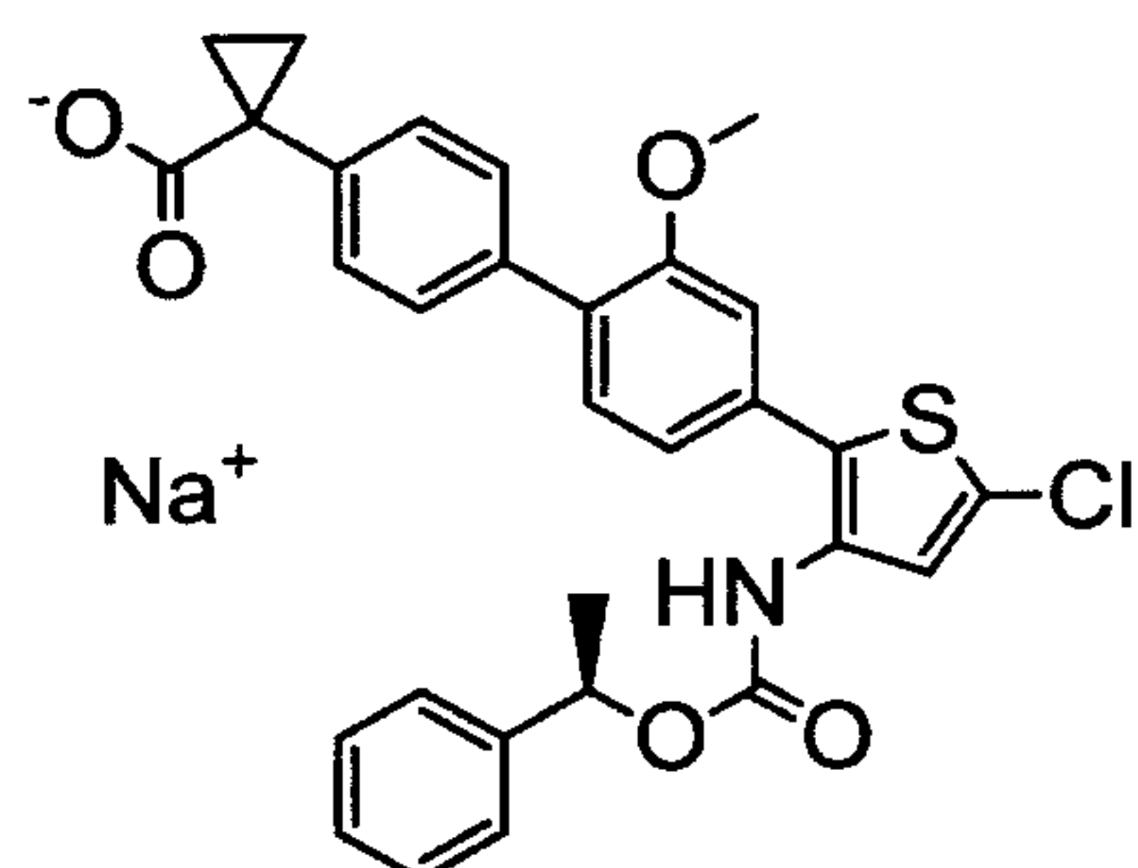
[Chem. 24]
