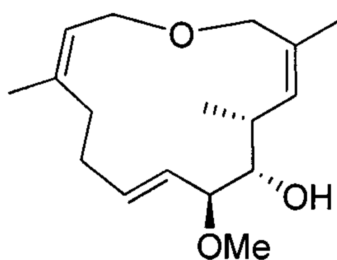
Methyl-cis-dehydromigraether ,
