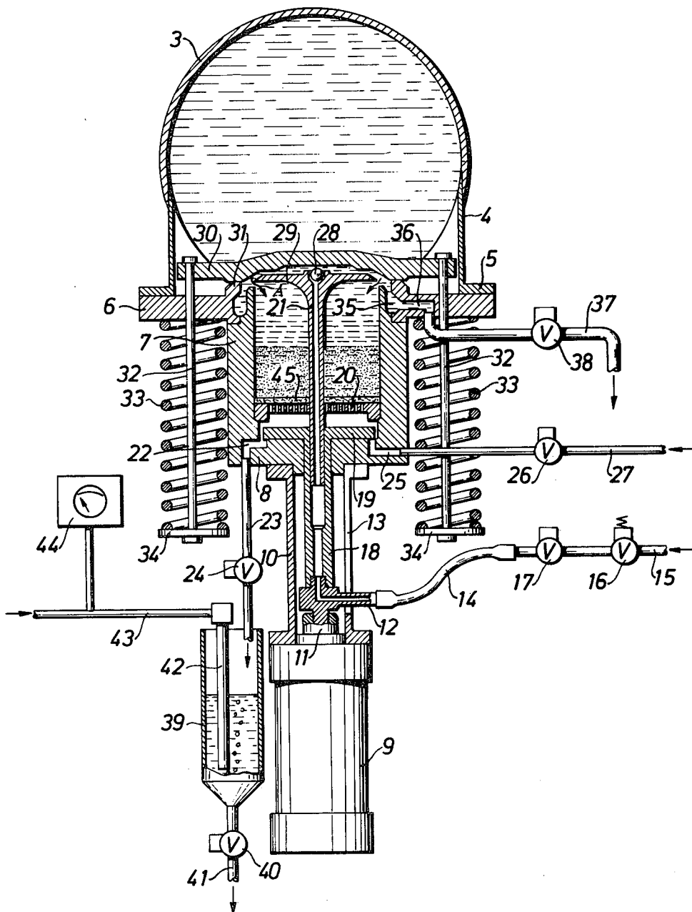
Fig. 1 (PRIOR ART)
