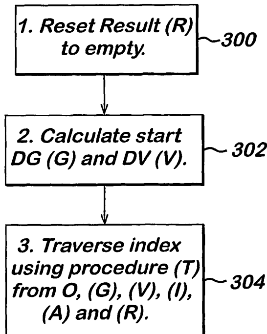
Fig. 11 Procedure (G) for Range Query with Min Key (I), Max Key (A) Returning Result (R)
