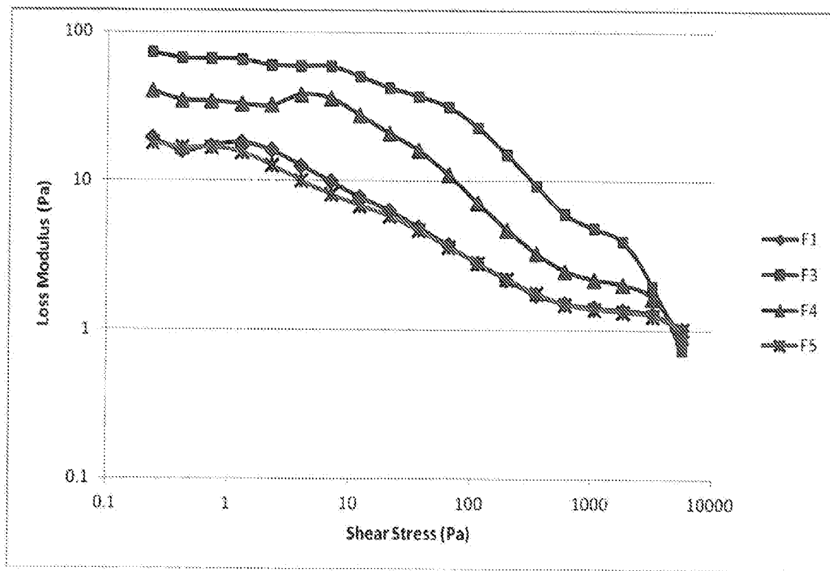
Figure 2. Loss Modulus vs. shear stress for model HIP emulsions
