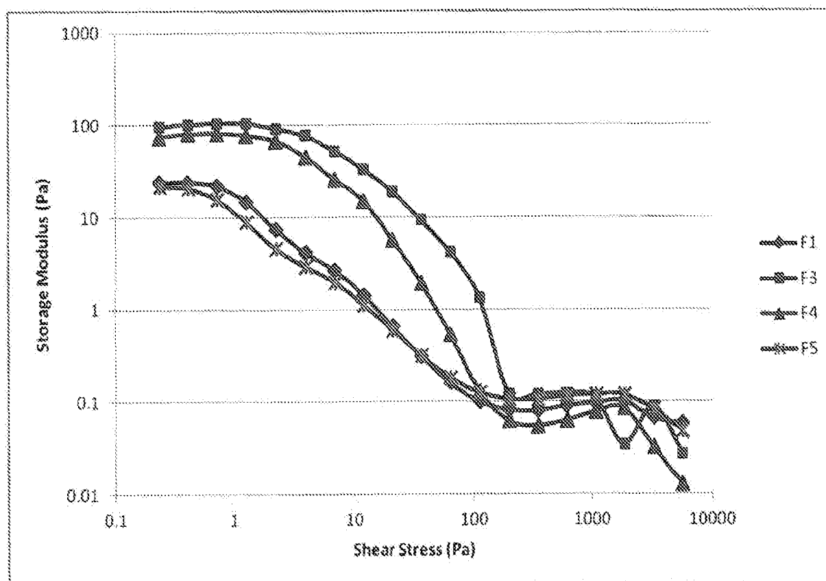
Figure 1. Storage Modulus vs. shear stress for model HIP emulsions
