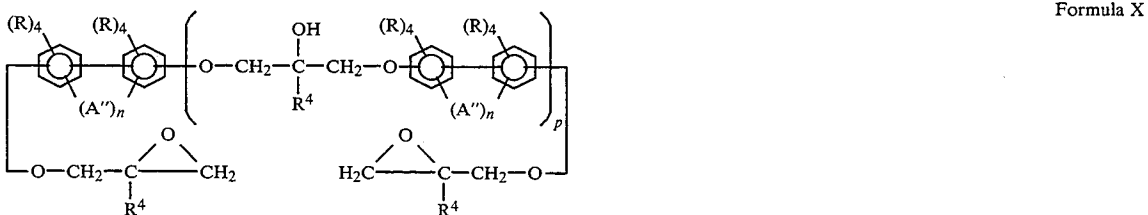
Formula XI
