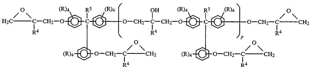
Formula VIII
