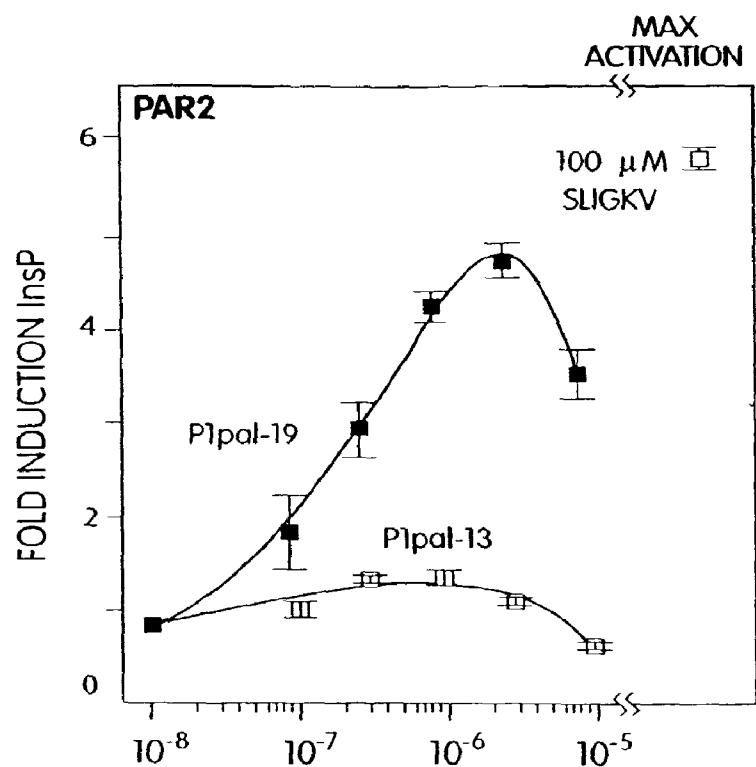
Fig. 6B [AGONIST] (M)
