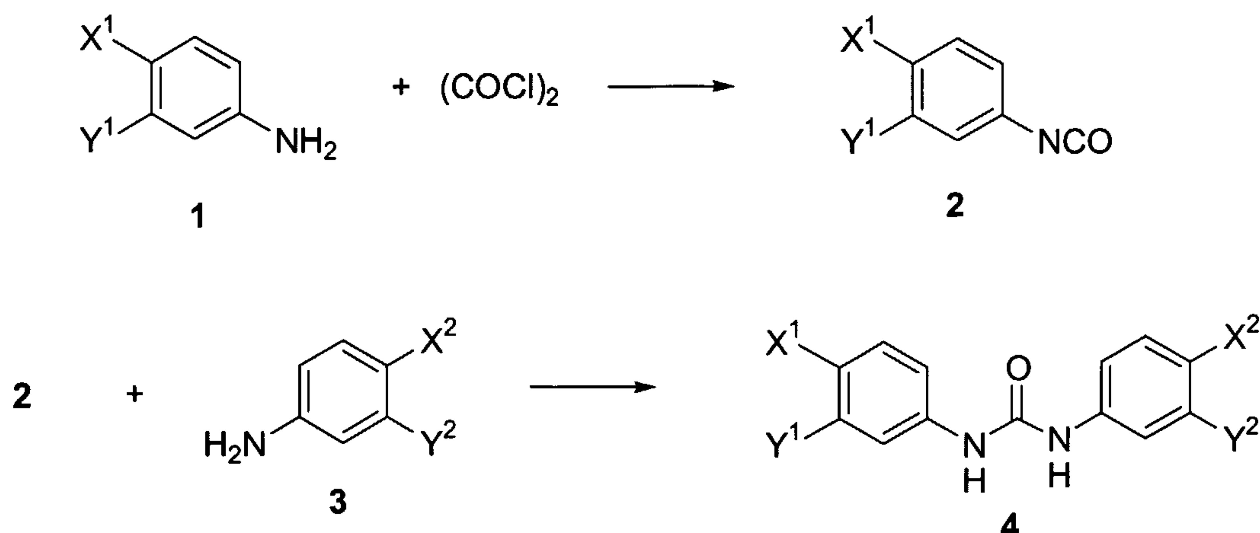
Reaction Scheme 1
