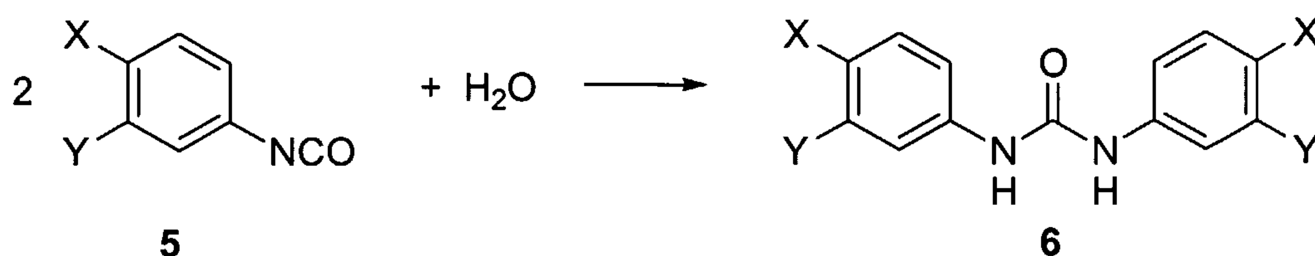
Reaction Scheme 2
