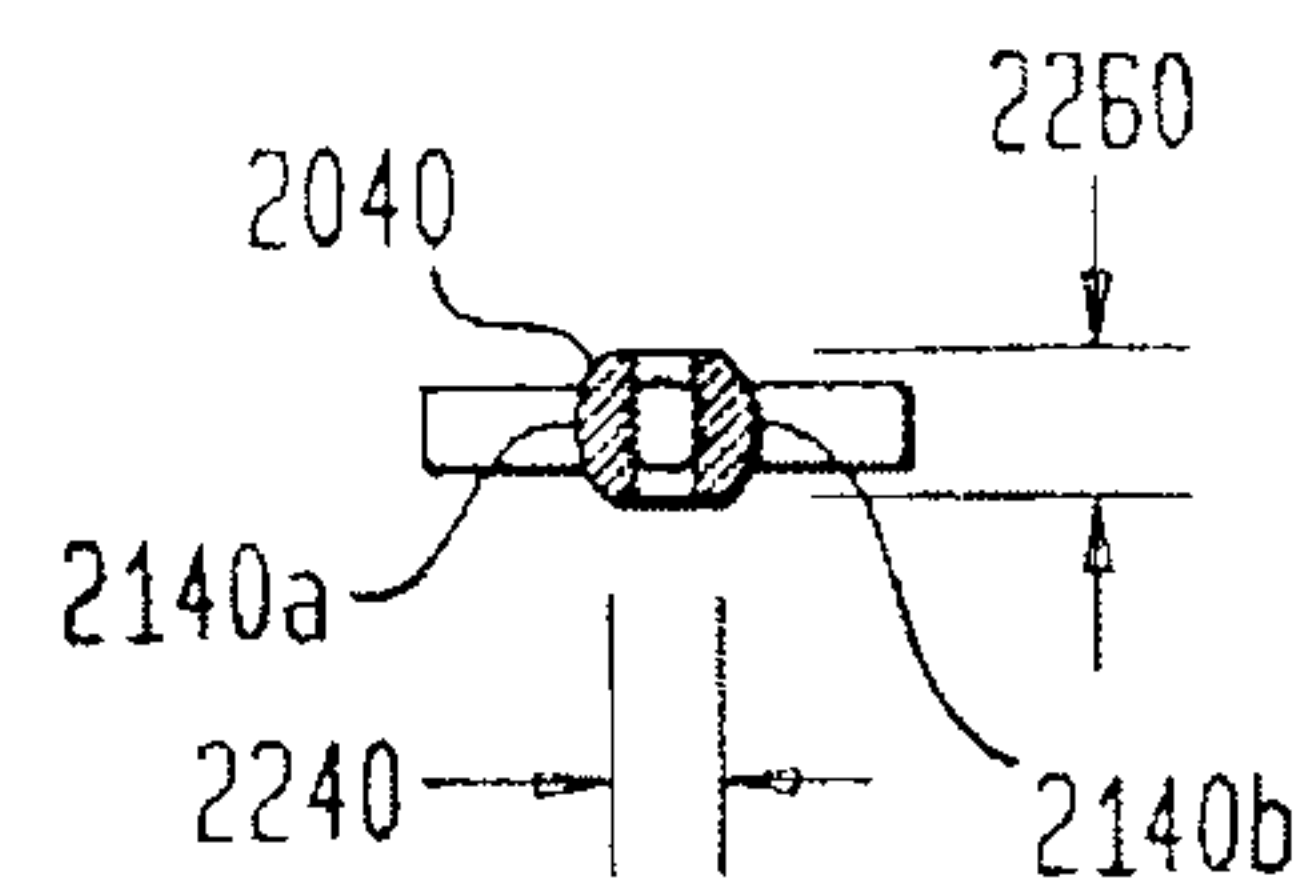
FIG. 2jj (SECTION C-C OF FIG. 2ii)
