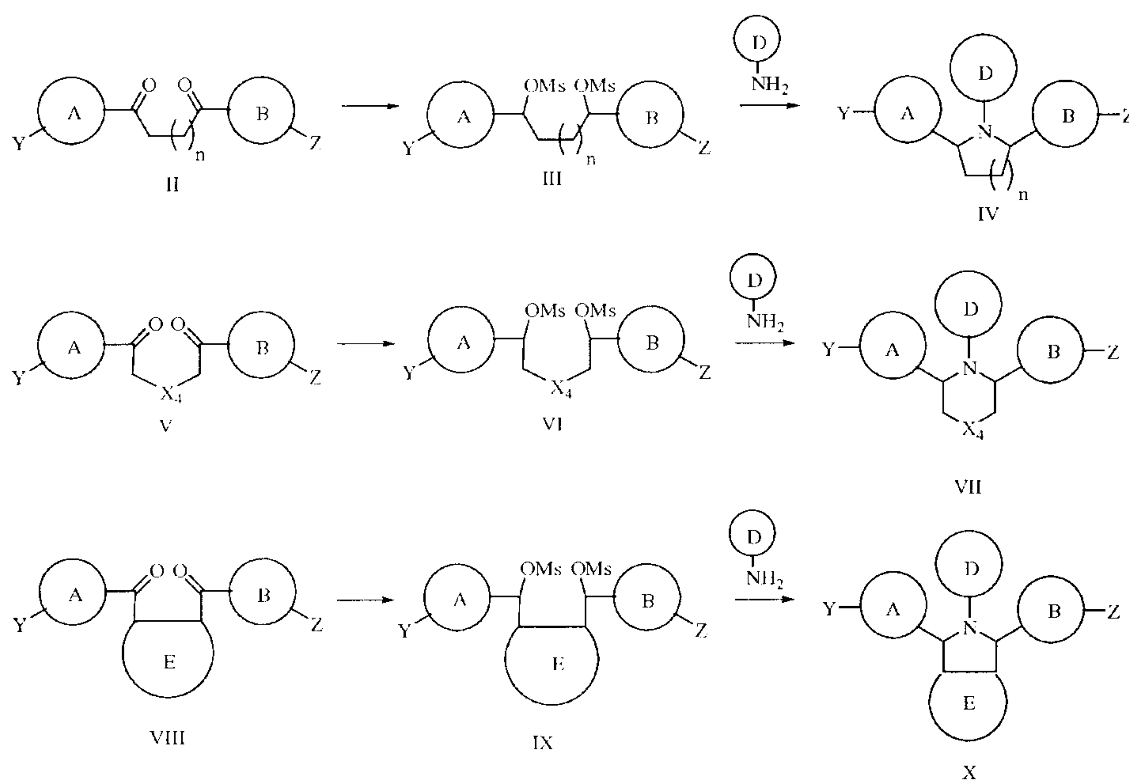
Scheme I
