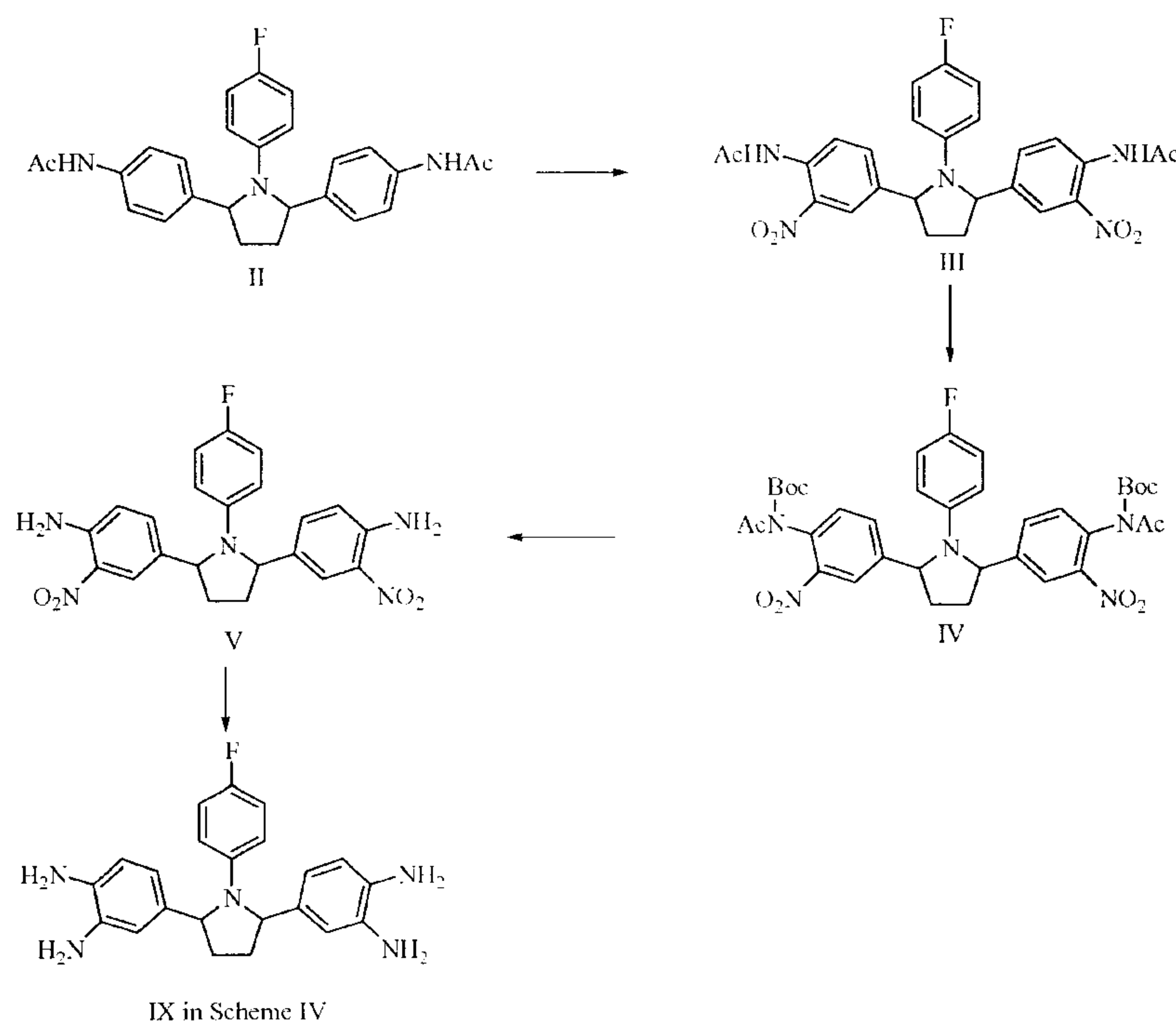
Scheme V
