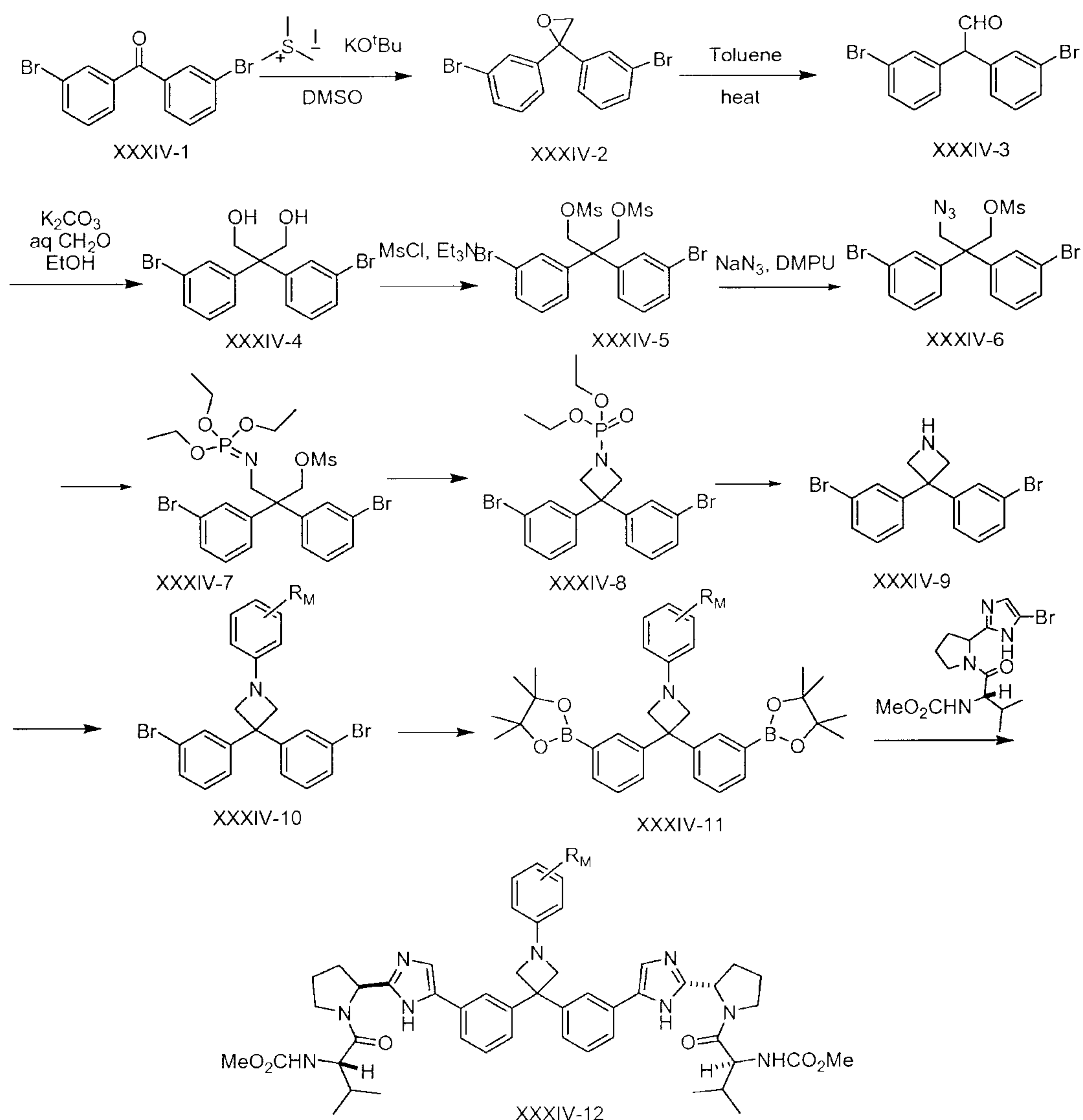
Scheme XXXIV
