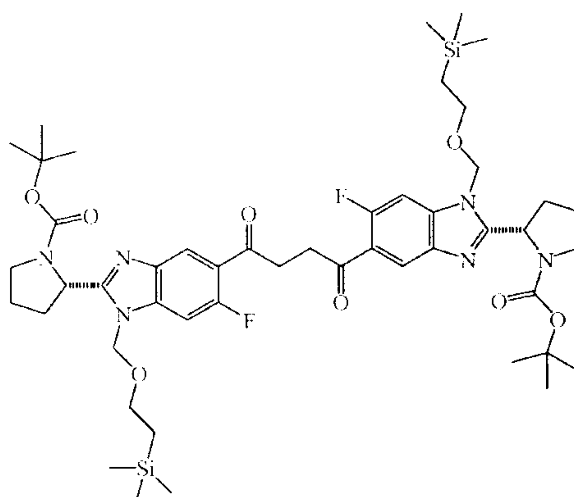
di- tert -butyl (2 S ,2' S )-2,2'-[(1,4-dioxobutane-1,4-diyl)bis(6-fluoro-1-{[2-(trimethylsilyl)ethoxy]methyl}-1 H -benzimidazole-5,2-diyl)]dipyrrolidine-1-carboxylate (ACD Name v12)
