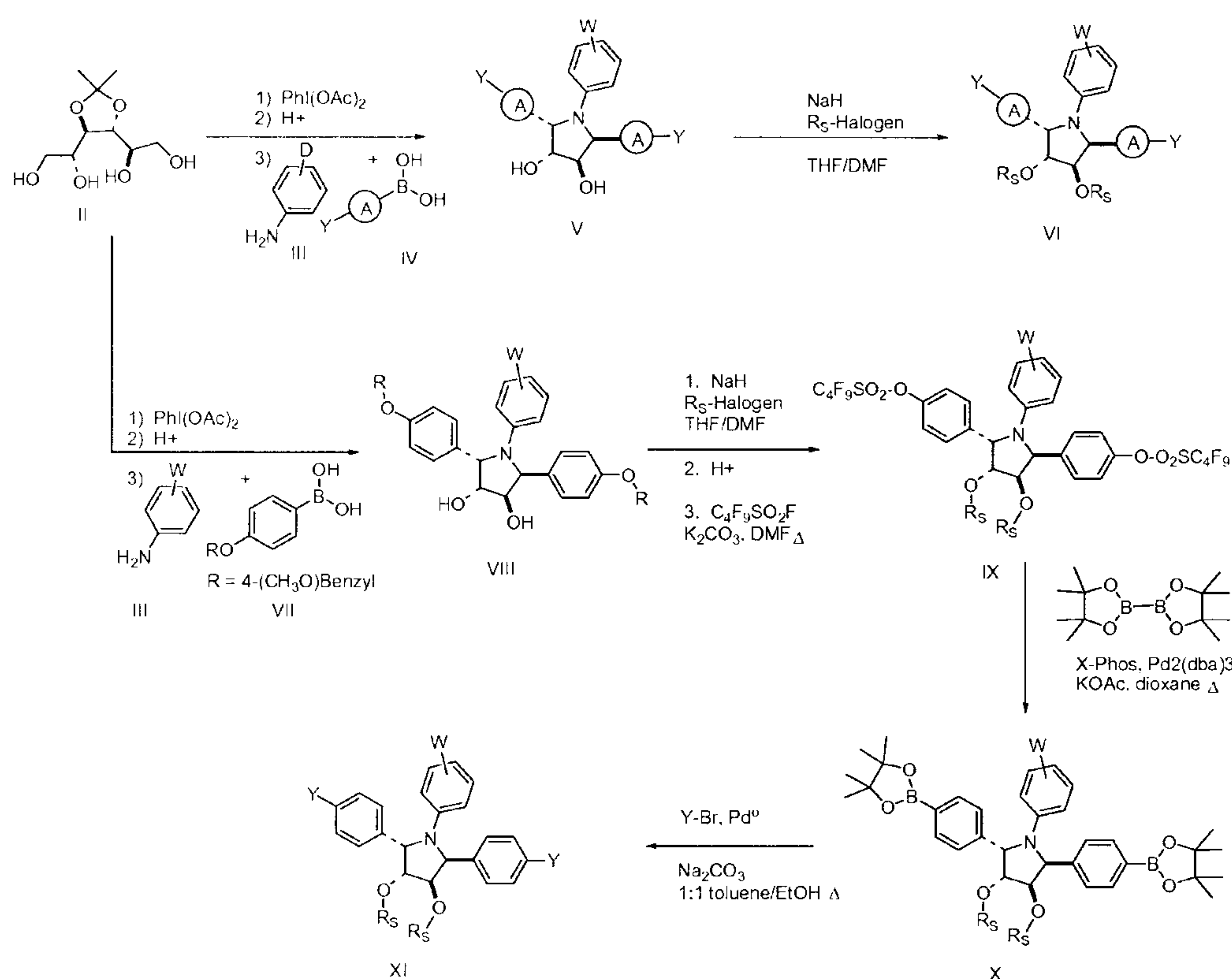
Scheme VIII
