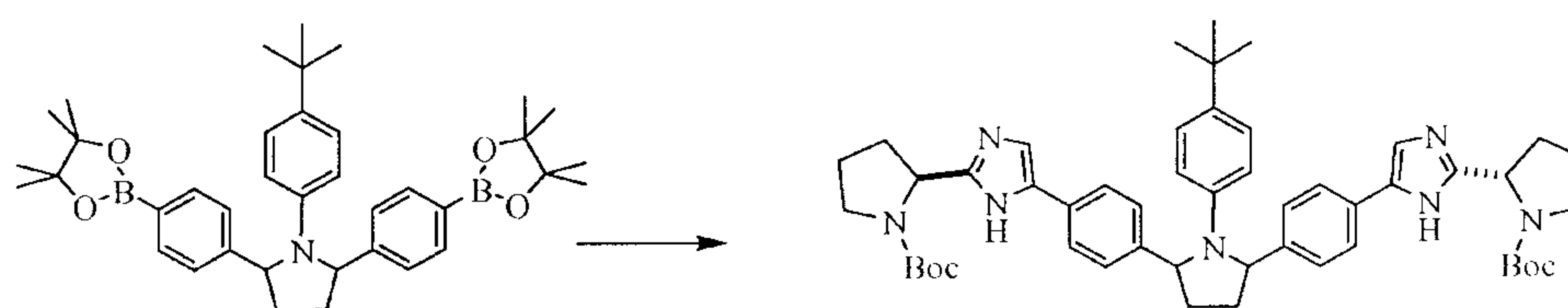
(2 S ,2' S )- tert -butyl 2,2'-(5,5'-(4,4'-(1-(4- tert -butylphenyl)pyrrolidine-2,5-diyl)bis(4,1-phenylene))bis(1 H -imidazole-5,2-diyl))dipyrrolidine-1-carboxylate
