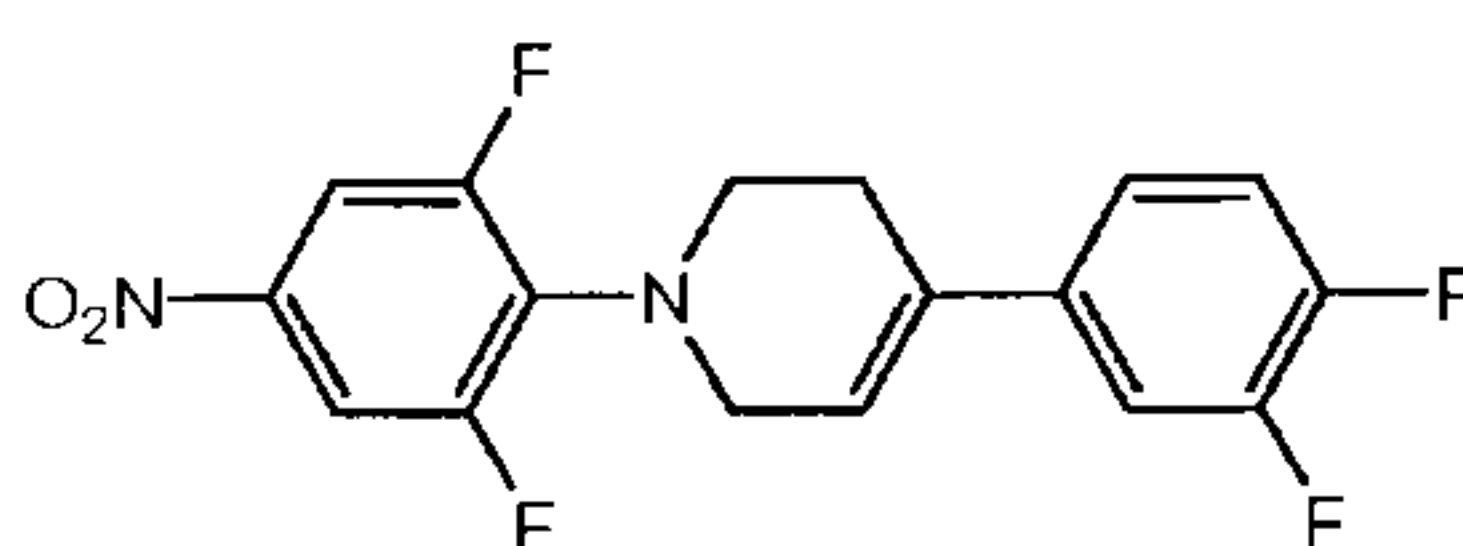
1-(2,6-difluoro-4-nitrophenyl)-4-(3,4-difluorophenyl)-1,2,3,6-tetrahydropyridine
