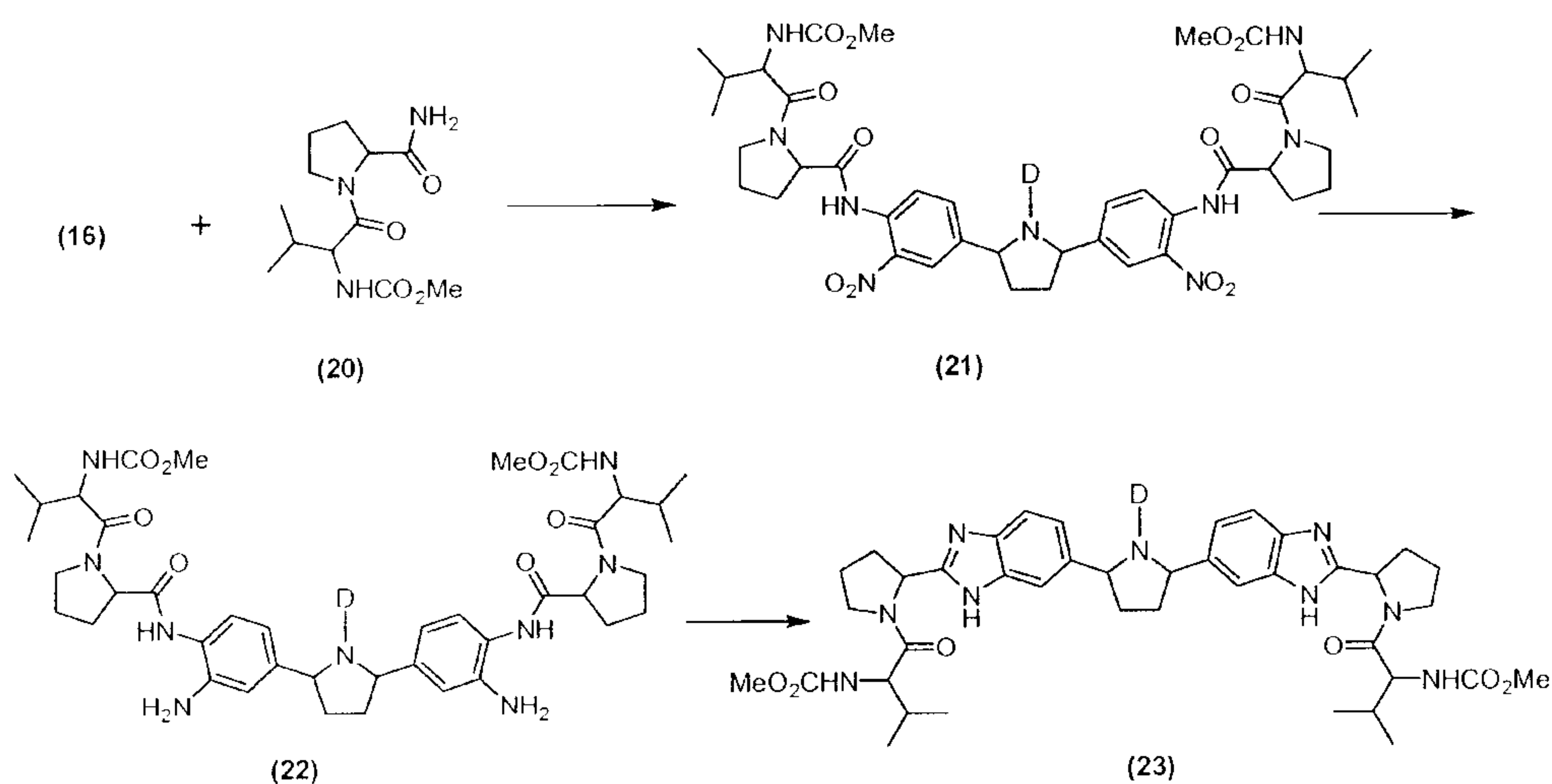
Scheme XIV
