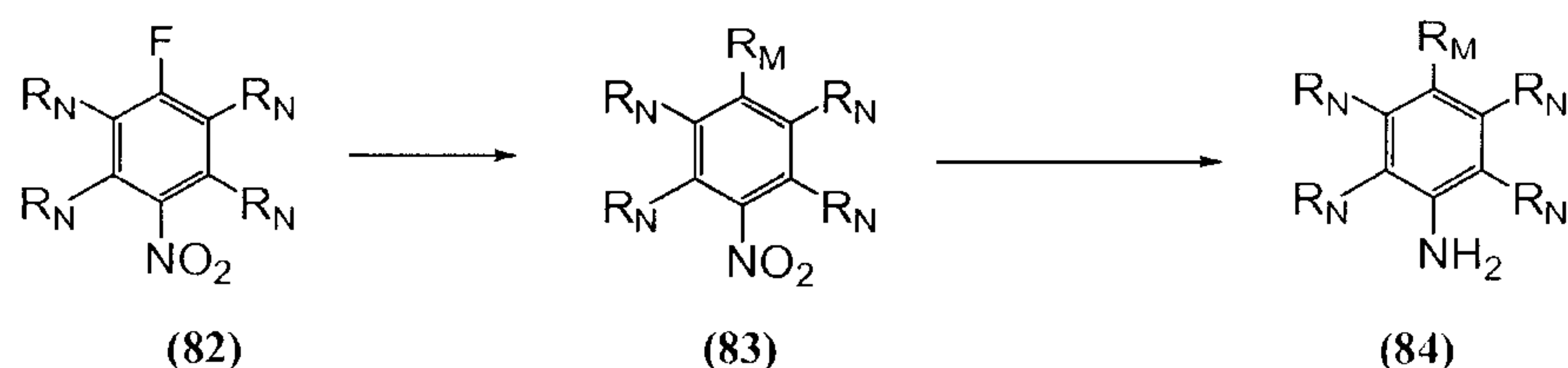
Scheme XXV
