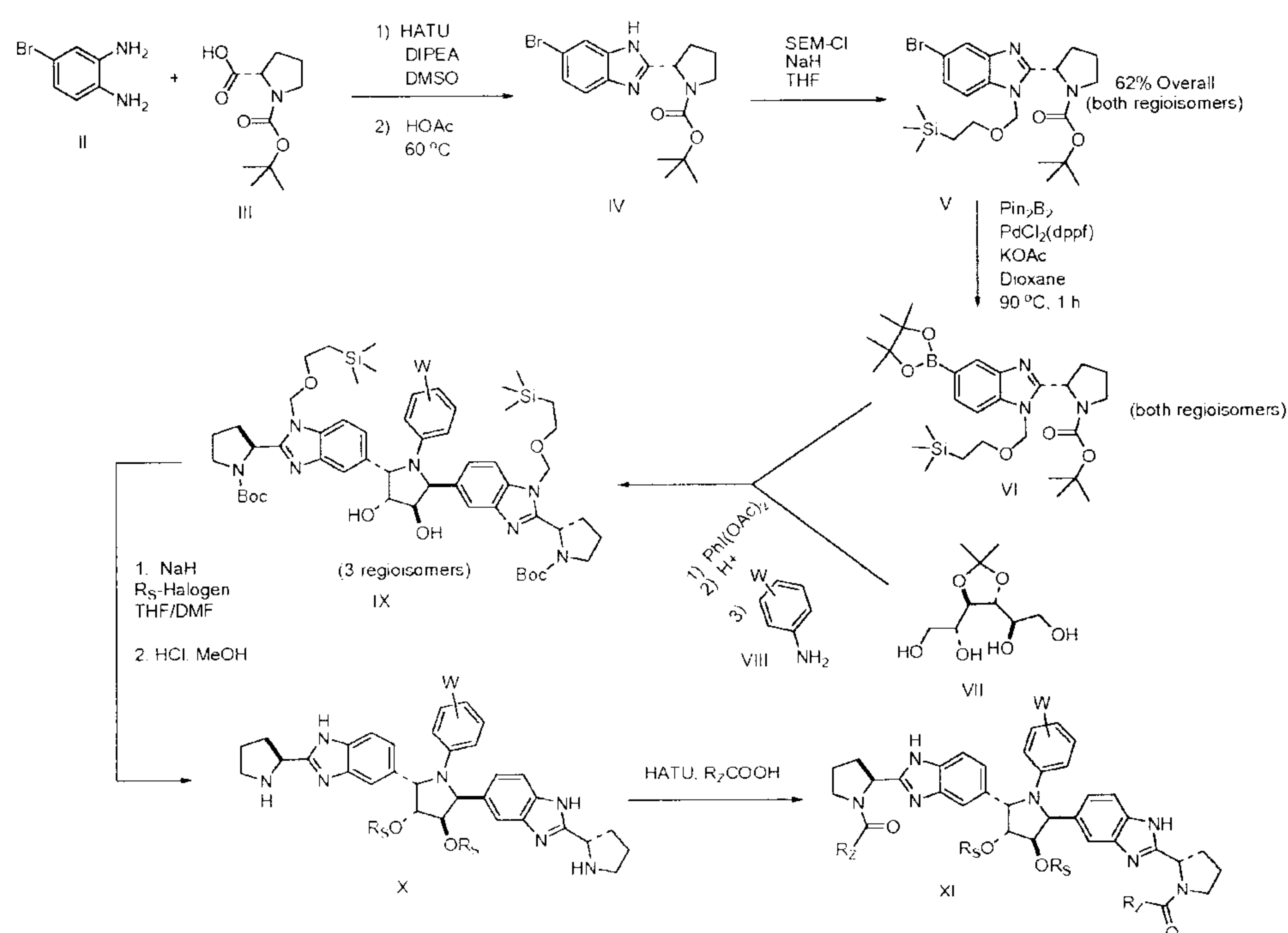
Scheme IX
