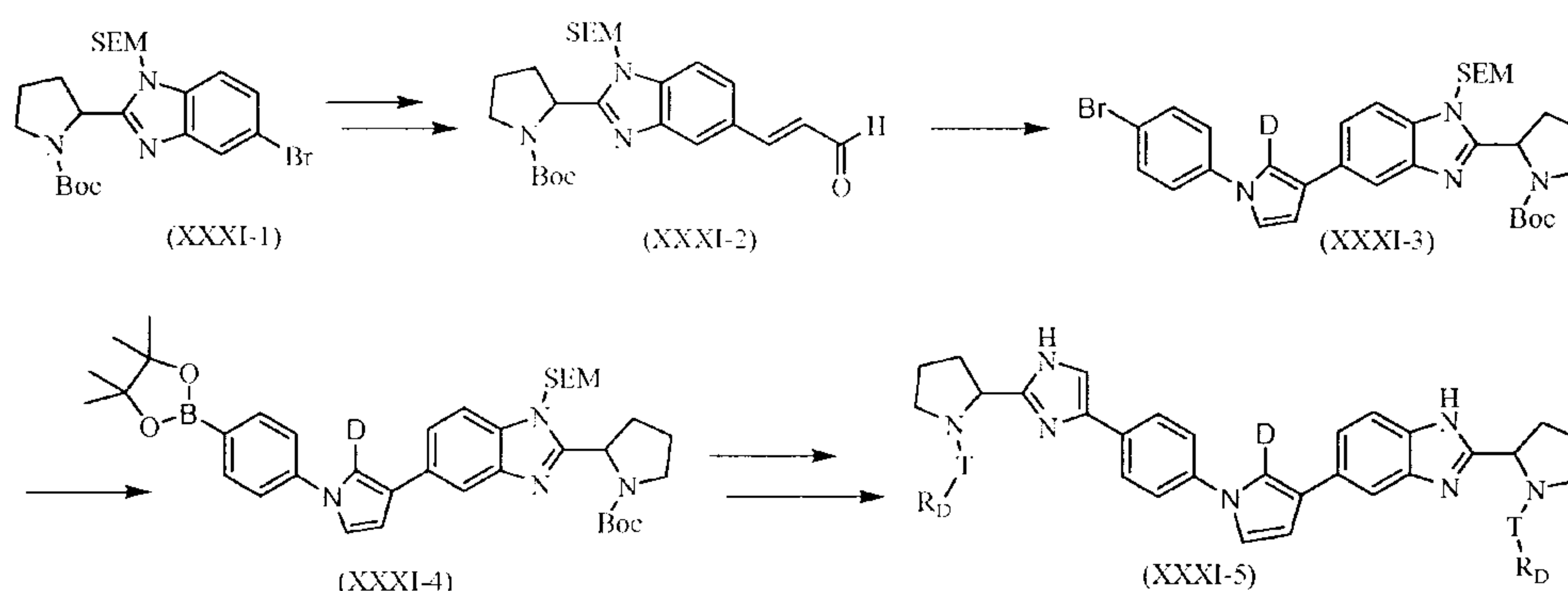
Scheme XXXI
