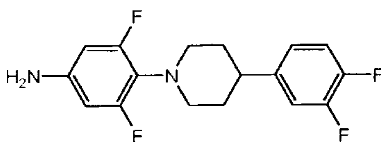
(4-(4-(3,4-difluorophenyl)piperidin-1-yl)-3,5-difluoroaniline
