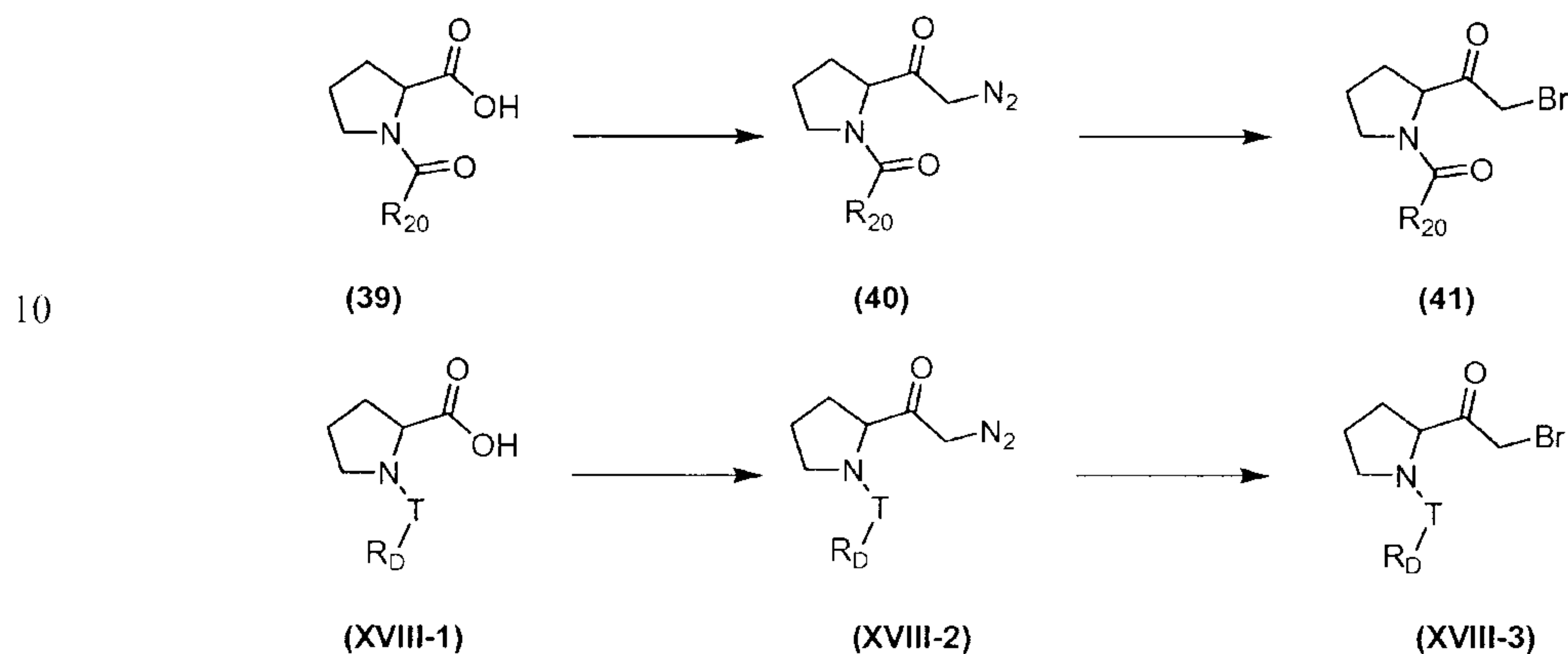
Scheme XVIII
