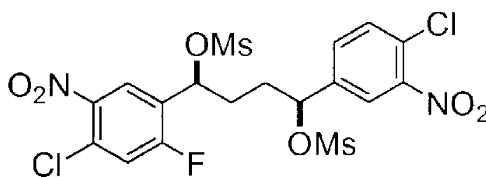
Intermediate 21
