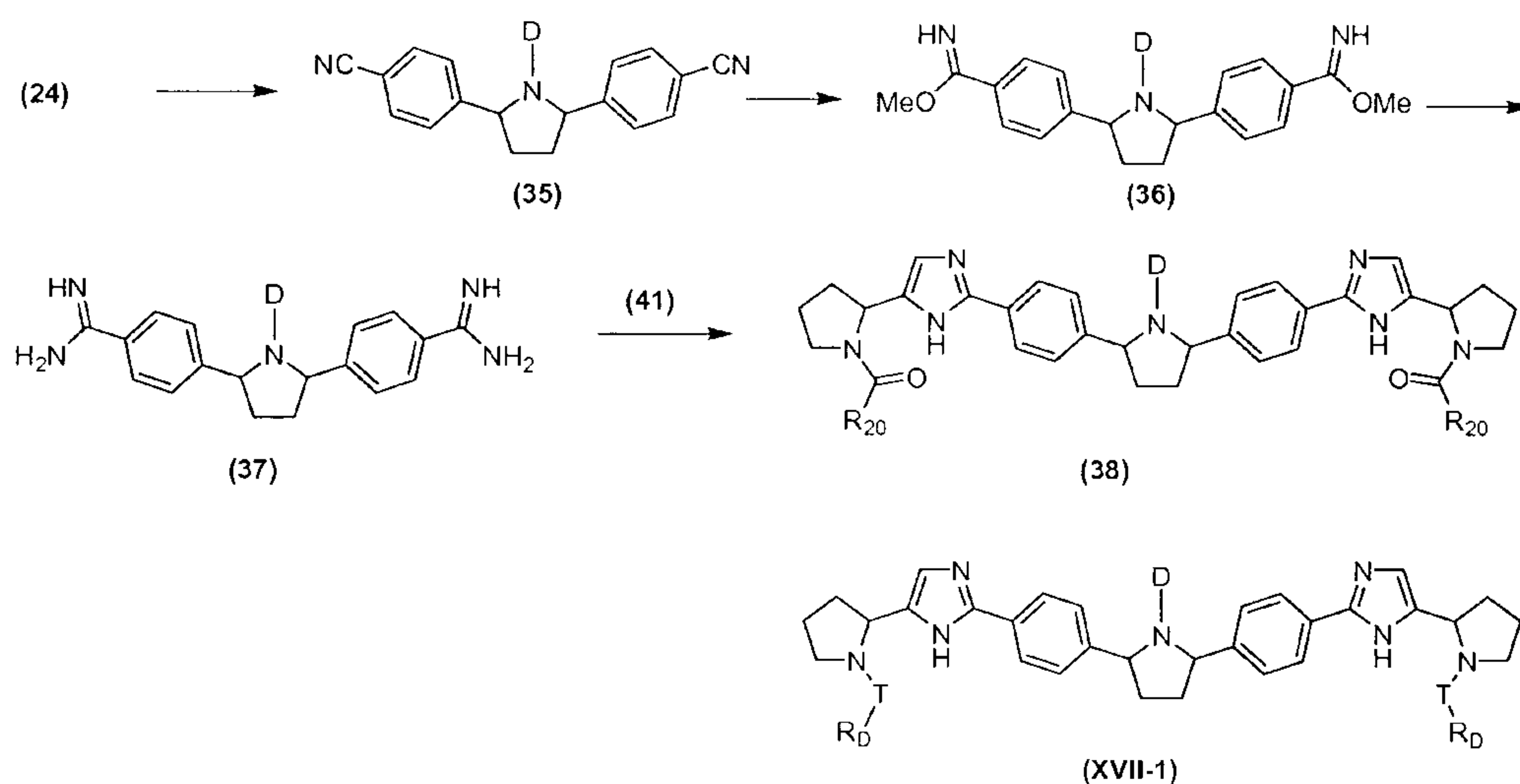
Scheme XVII
