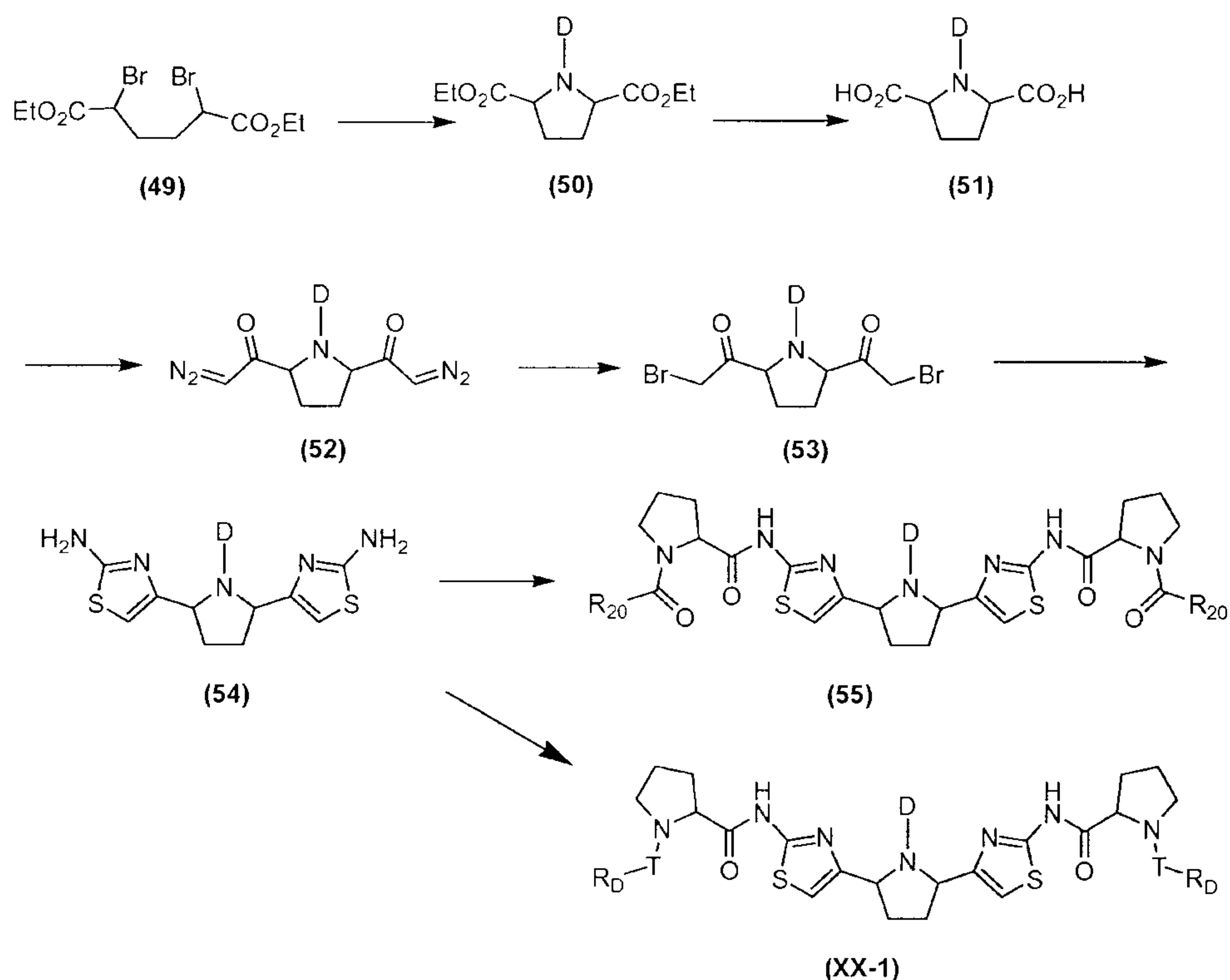
Scheme XX
