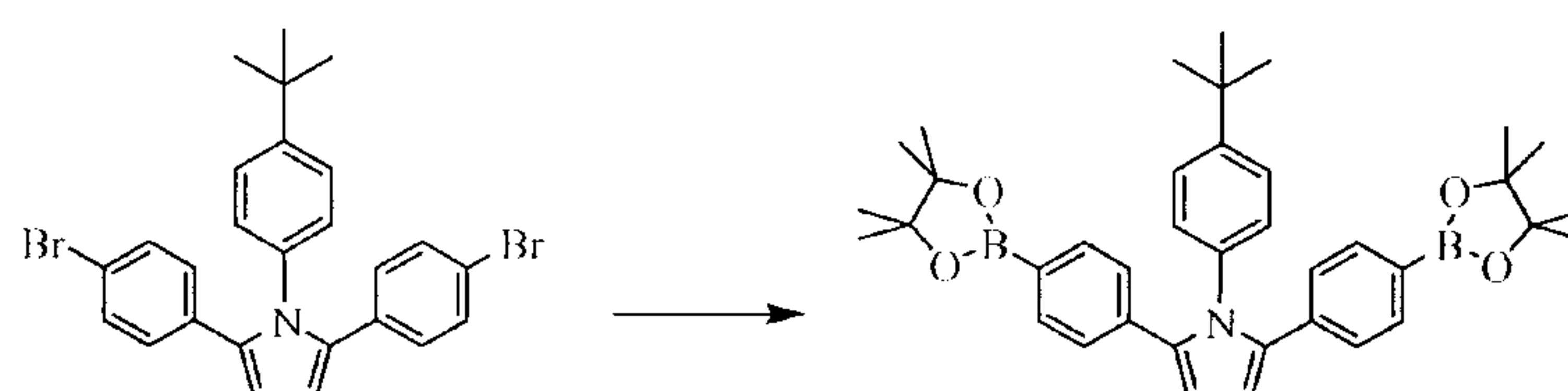
1-(4- tert -butylphenyl)-2,5-bis(4-(4,4,5,5-tetramethyl-1,3,2-dioxaborolan-2-yl)phenyl)-1 H -pyrrole
