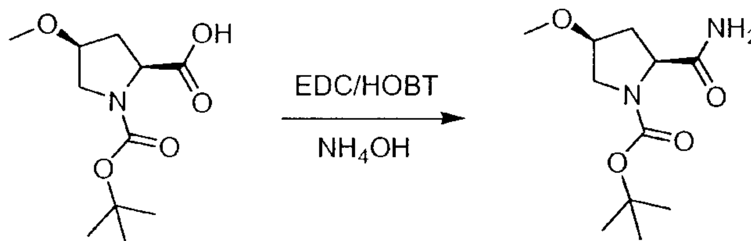
(2 S ,4 S )- tert -butyl 2-carbamoyl-4-methoxypyrrolidine-1-carboxylate
