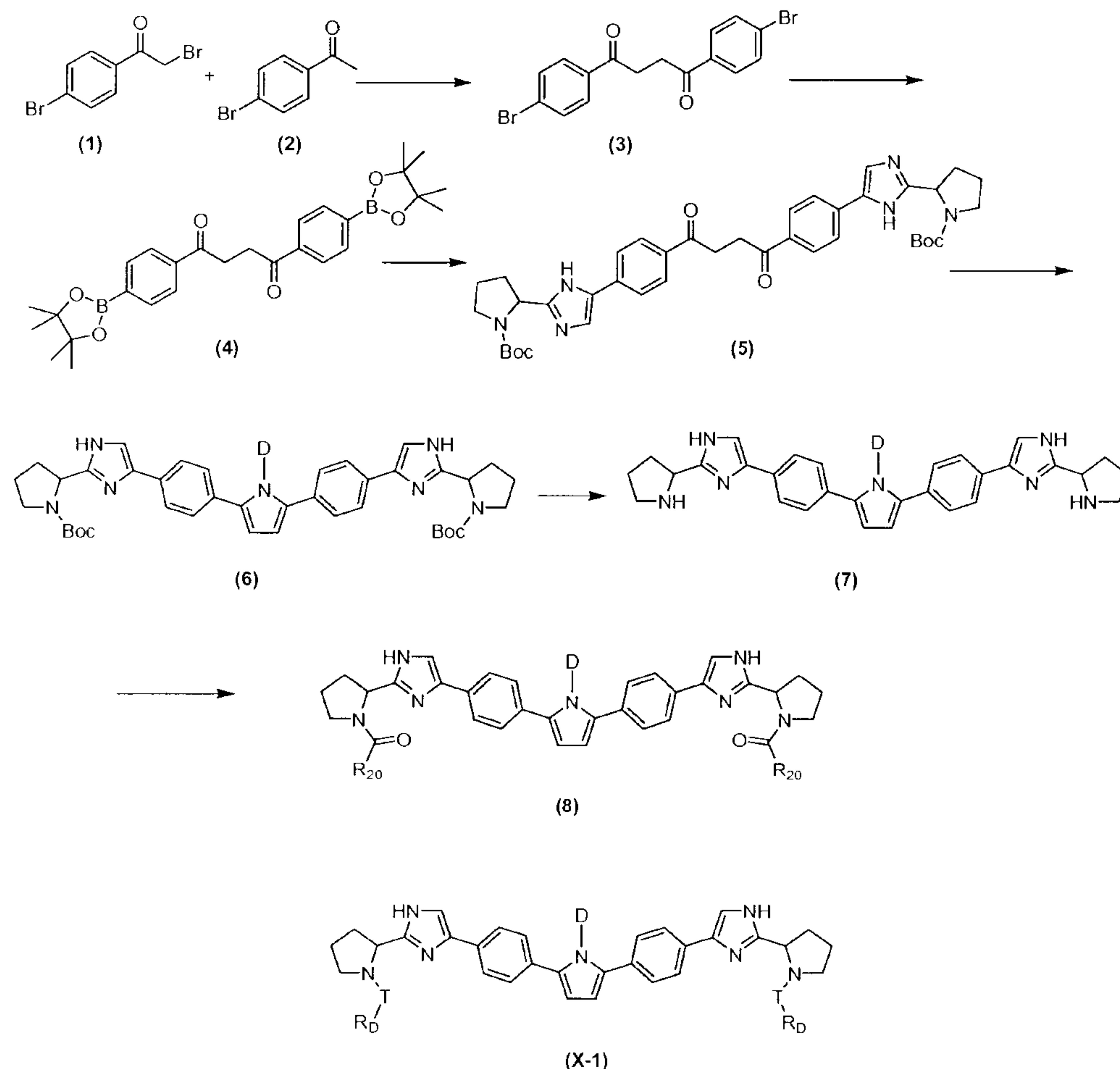
Scheme X
