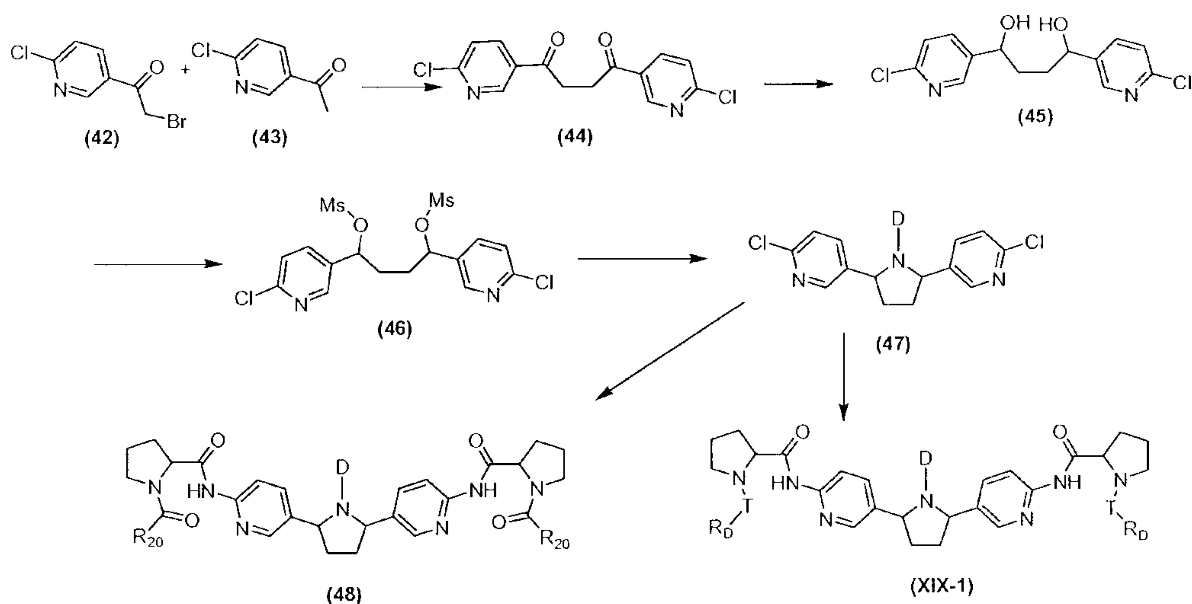
Scheme XIX
