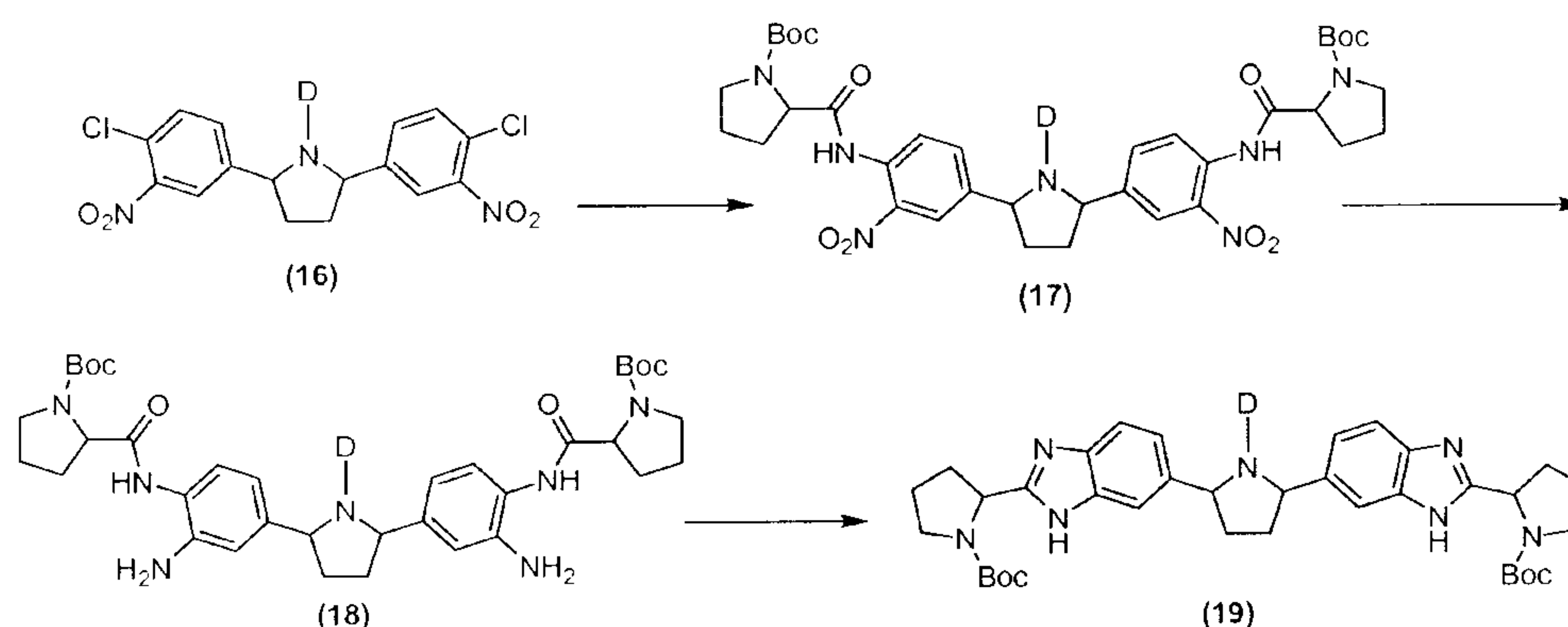
Scheme XIII
