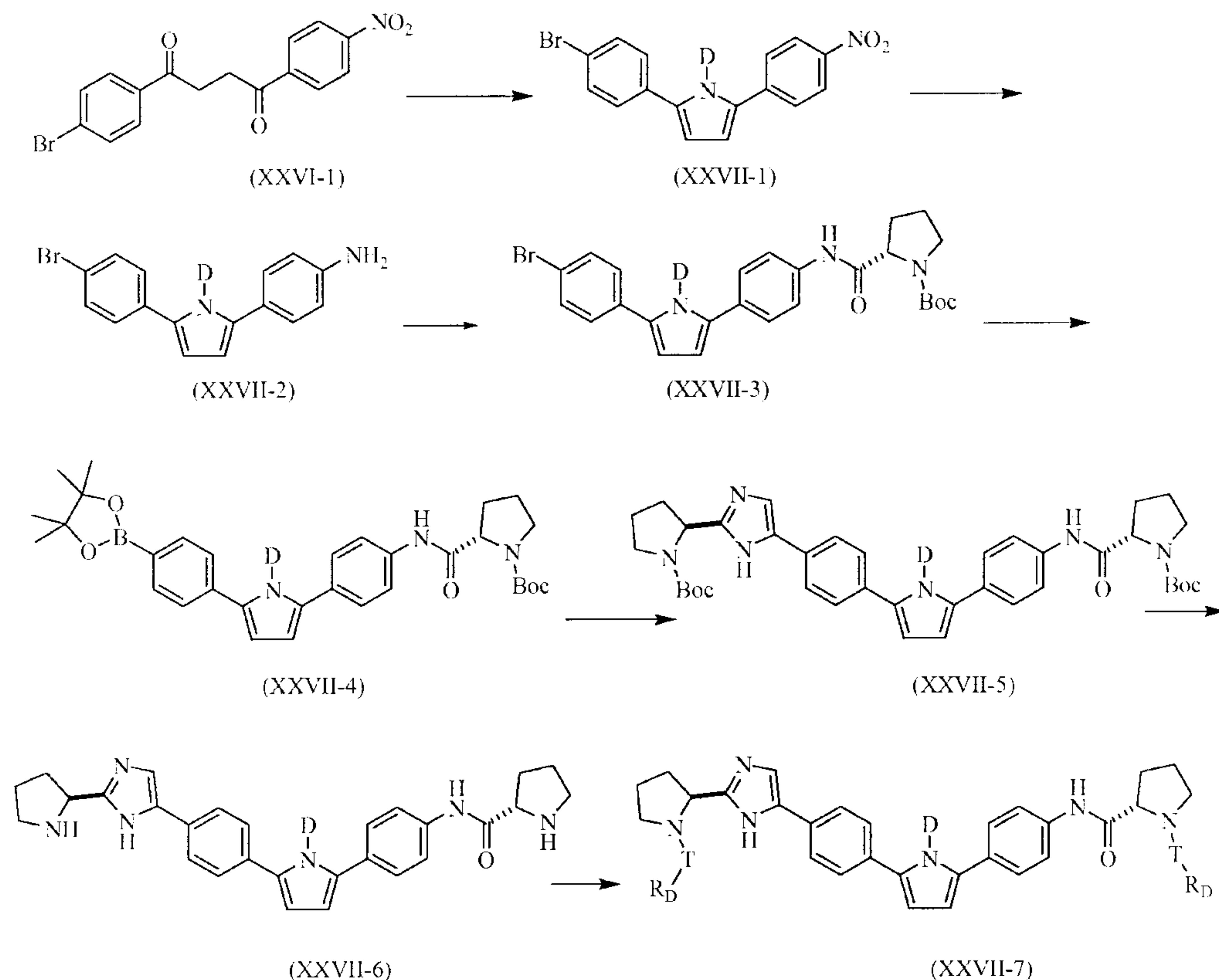
Scheme XXVII
