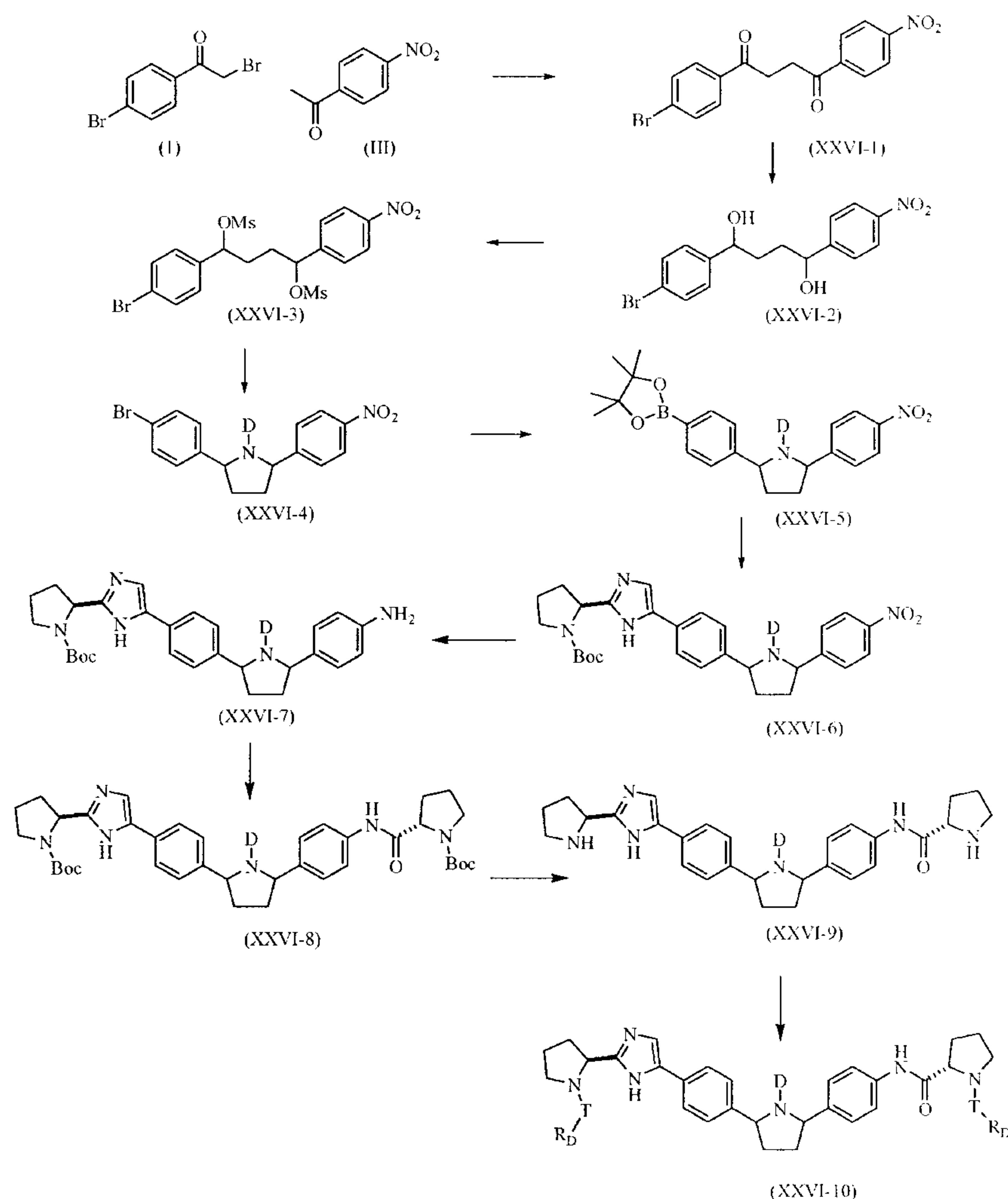
Scheme XXVI
