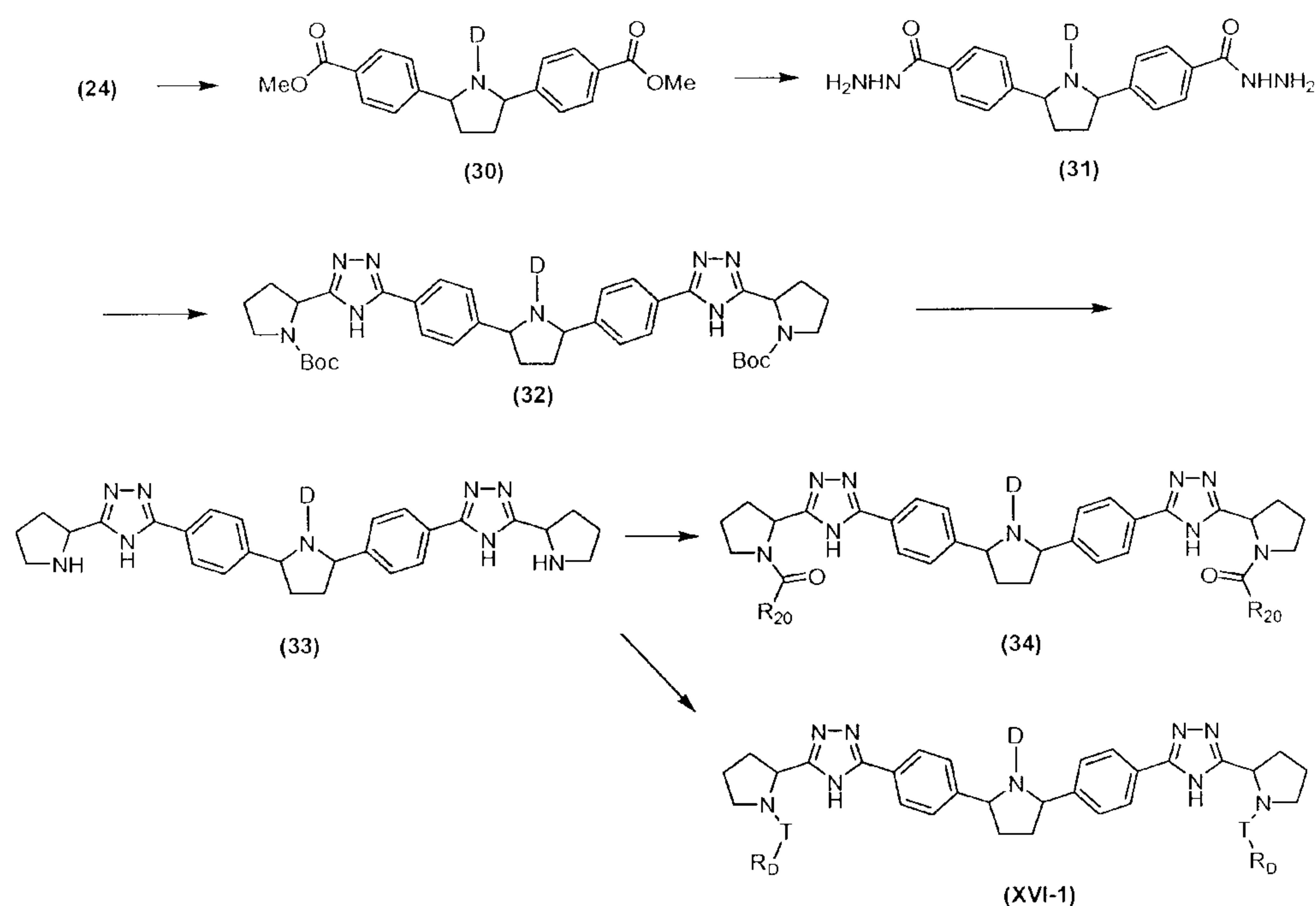
Scheme XVI
