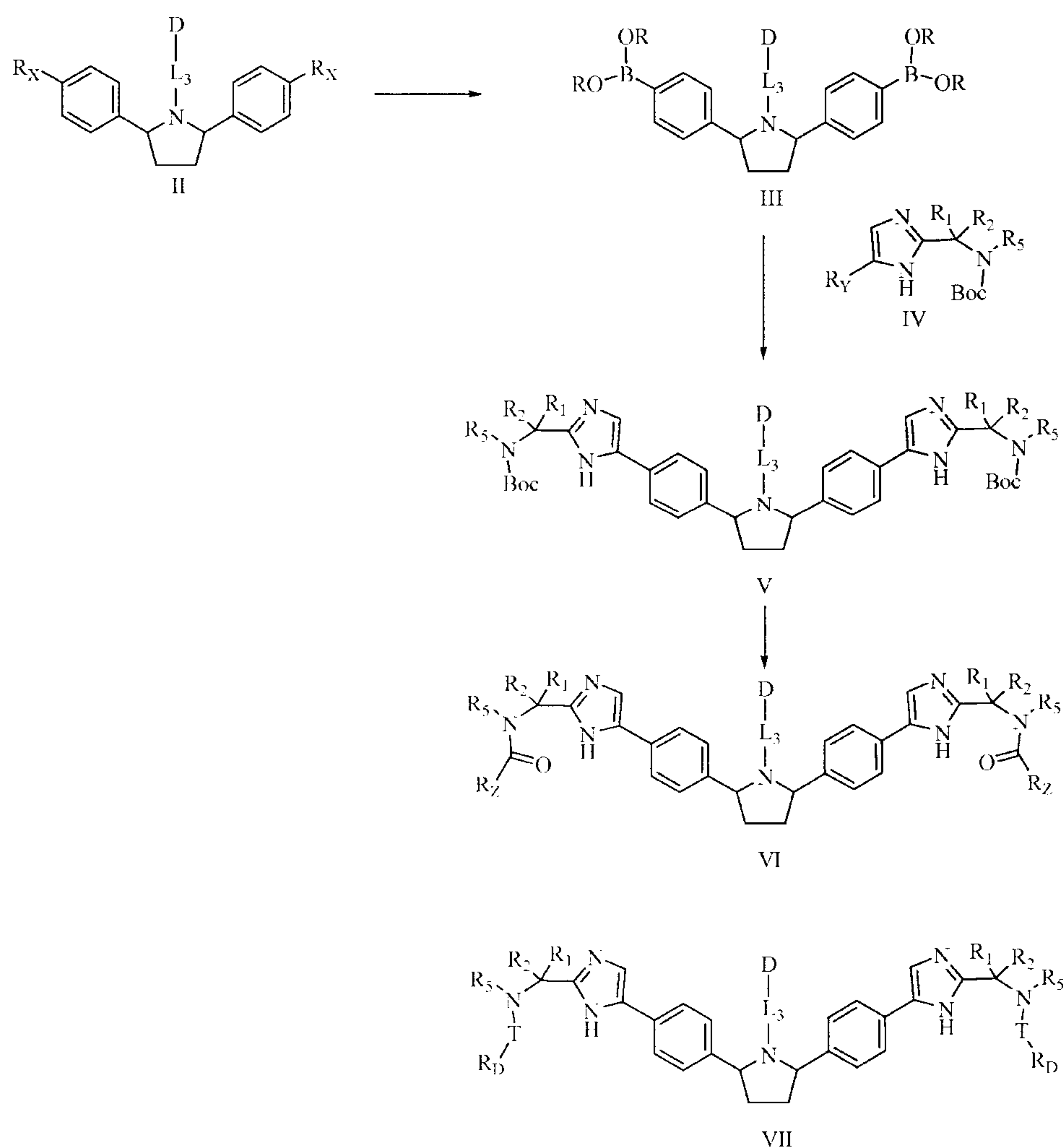
Scheme VII
