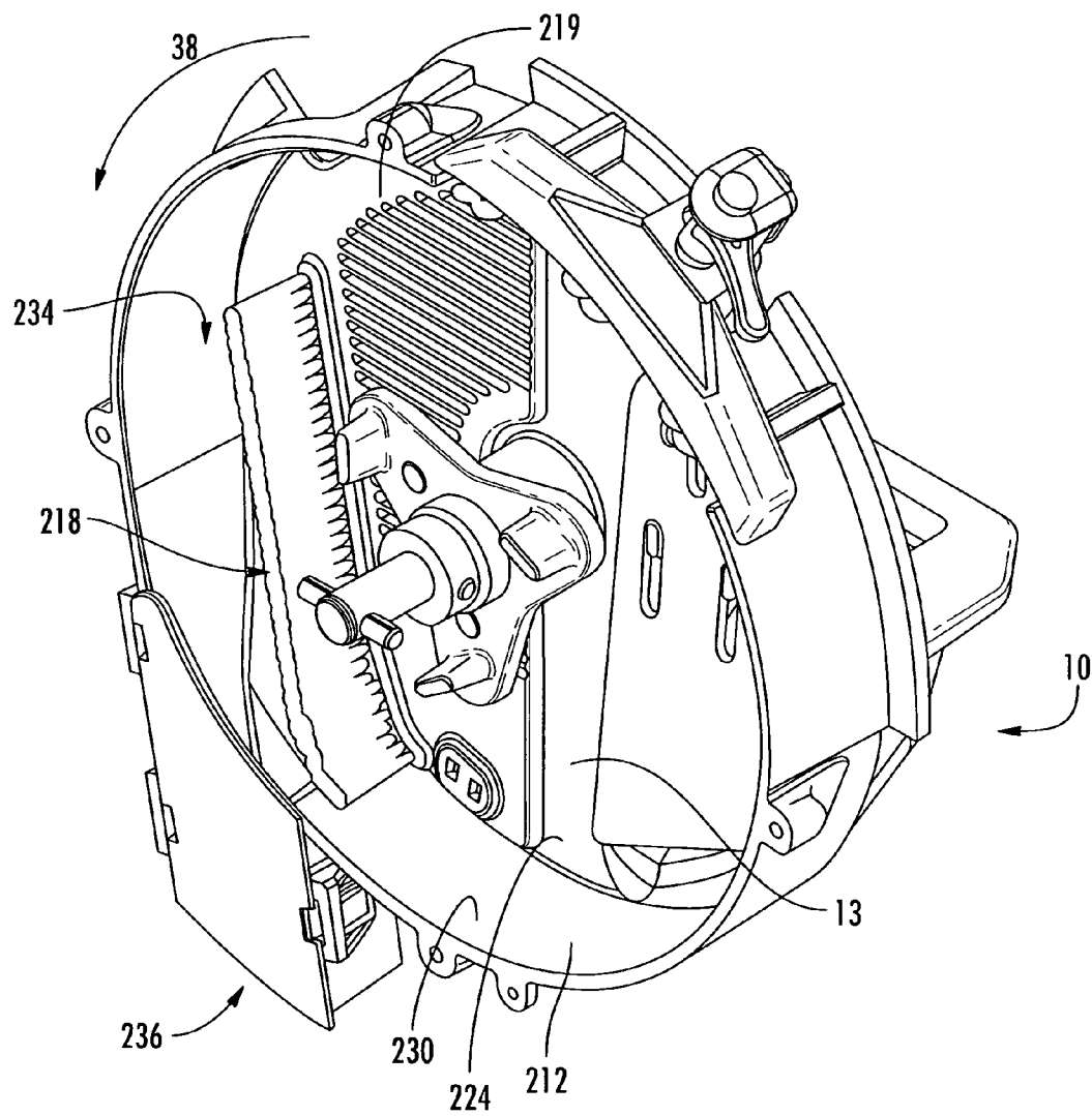
FIG. 4 (PRIOR ART)
