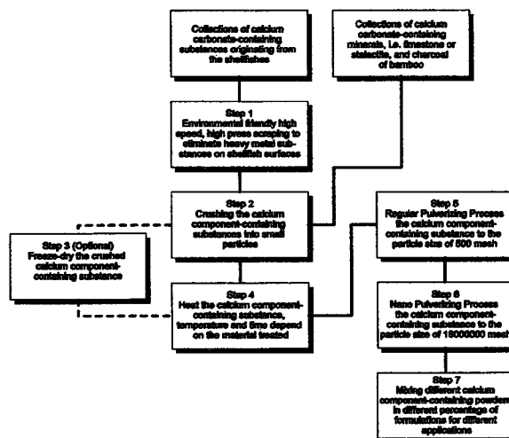
Flow chart of producing acid-neutralizing agent
