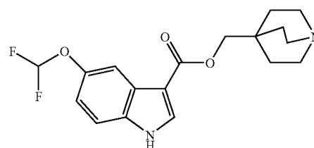
(15): quinuclidin-4-ylmethyl 5-(difluoromethoxy)-1H-indole-3-carboxylate;
