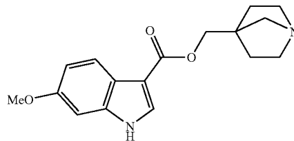
(25): 1-azabicyclo[2.2.1]heptan-4-ylmethyl 6-methoxy-1H-indole-3-carboxylate;
