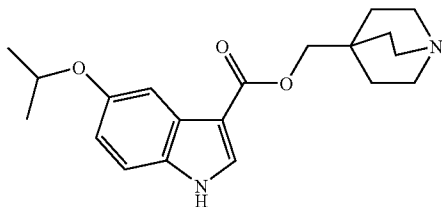
(18): quinuclidin-4-ylmethyl 5-isopropoxy-1H-indole-3-carboxylate;
