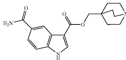
(8): quinuclidin-4-ylmethyl 5-carbamoyl-1H-indole-3-carboxylate;
