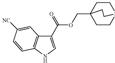
(7): quinuclidin-4-ylmethyl 5-cyano-1H-indole-3-carboxylate;
