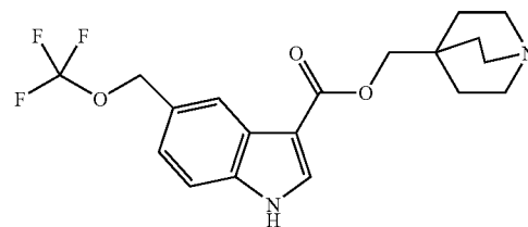
(17): quinuclidin-4-ylmethyl 5-((trifluoromethoxy)methyl)-1H-indole-3-carboxylate;
