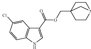
(22): 1-azabicyclo[2.2.1]heptan-4-ylmethyl 5-chloro-1H-indole-3-carboxylate;
