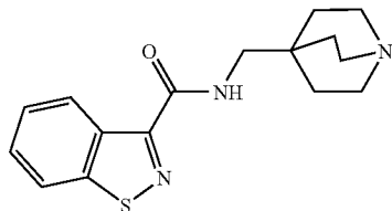
(5): N-(quinuclidin-4-ylmethyl)benzo[d]isothiazole-3-carboxamide;
