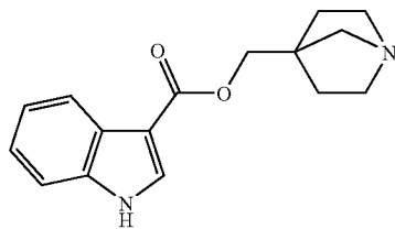
(20): 1-azabicyclo[2.2.1]heptan-4-ylmethyl 1H-indole-3-carboxylate;
