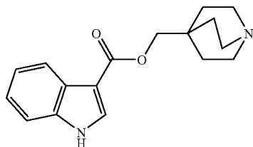
(2): quinuclidin-4-ylmethyl 1H-indole-3-carboxylate;
