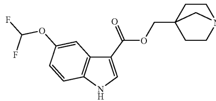
(24): 1-azabicyclo[2.2.1]heptan-4-ylmethyl 5-(dif- luoromethoxy)-1H-indole-3-carboxylate;
