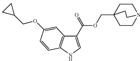
(19): quinuclidin-4-ylmethyl 5-(cyclopropyl- methoxy)-1H-indole-3-carboxylate;
