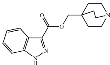
(12): quinuclidin-4-ylmethyl 1H-indazole-3-carboxylate;
