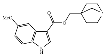
(23): 1-azabicyclo[2.2.1]heptan-4-ylmethyl 5-methoxy-1H-indole-3-carboxylate;
