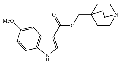
(13): quinuclidin-4-ylmethyl 5-methoxy-1H-indole-3-carboxylate;
