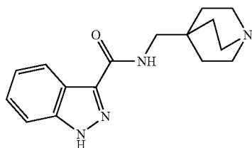
(3): N-(quinuclidin-4-ylmethyl)-1H-indazole-3-carboxamide;
