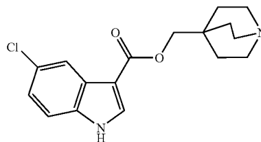
(6): quinuclidin-4-ylmethyl 5-chloro-1H-indole-3-carboxylate;
