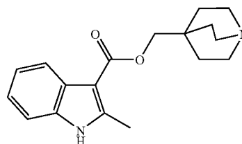
(9): quinuclidin-4-ylmethyl 2-methyl-1H-indole-3-carboxylate;
