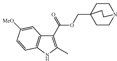
(10): quinuclidin-4-ylmethyl 5-methoxy-2-methyl-1H-indole-3-carboxylate;
