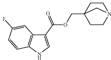
(21): 1-azabicyclo[2.2.1]heptan-4-ylmethyl 5-fluoro-1H-indole-3-carboxylate;
