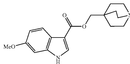
(14): quinuclidin-4-ylmethyl 6-methoxy-1H-indole-3-carboxylate;
