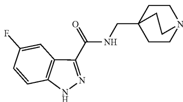
(4): 5-fluoro-N-(quinuclidin-4-ylmethyl)-1H-indazole-3-carboxamide;
