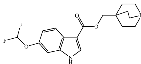
(16): quinuclidin-4-ylmethyl 6-(difluoromethoxy)-1H-indole-3-carboxylate;
