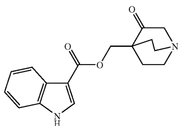
(11): (3-oxoquinuclidin-4-yl)methyl 1H-indole-3-carboxylate;
