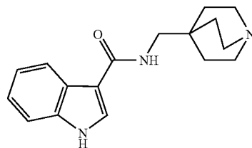
(1): quinuclidin-4-ylmethyl 1H-indole-3-carboxamide;
