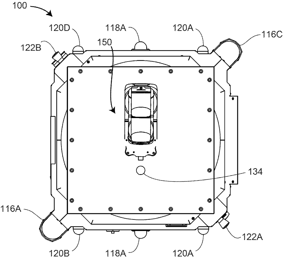
TOP VIEW FIG. 1D
