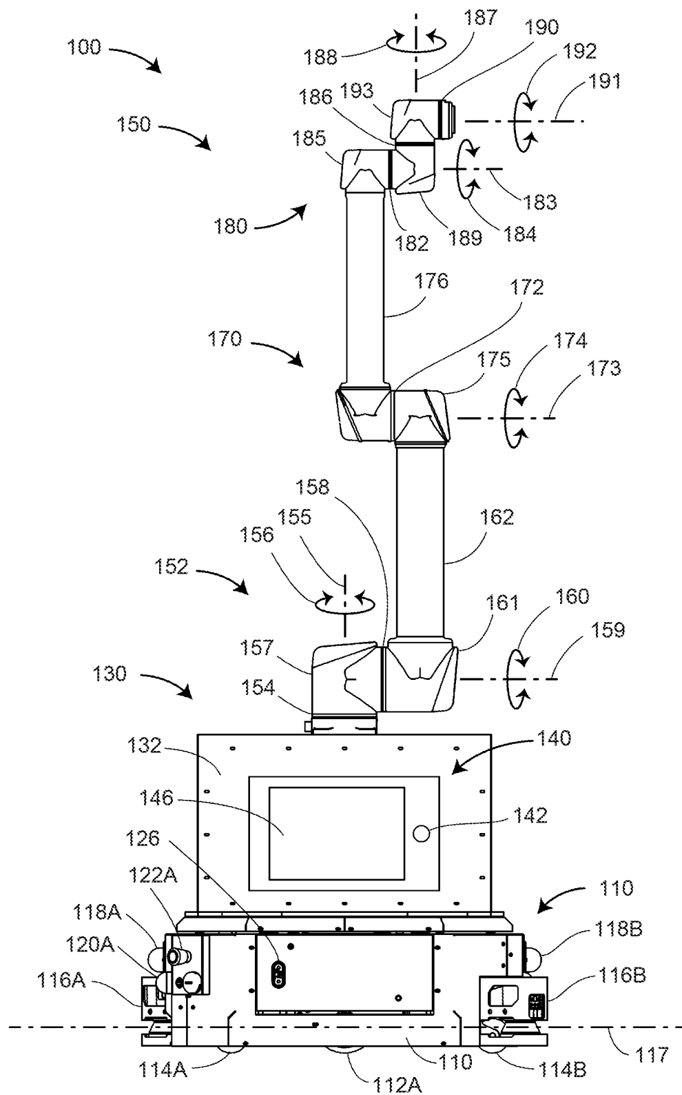
RIGHT SIDE VIEW FIG. 1B
