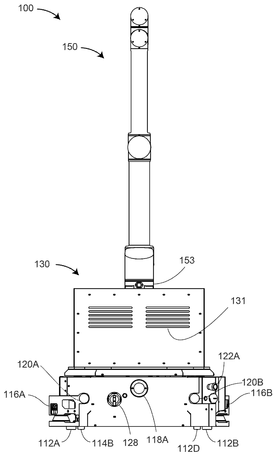
FRONT VIEW FIG. 1C
