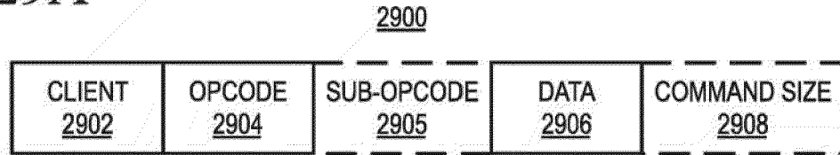
FIG. 29A GRAPHICS PROCESSOR COMMAND FORMAT
