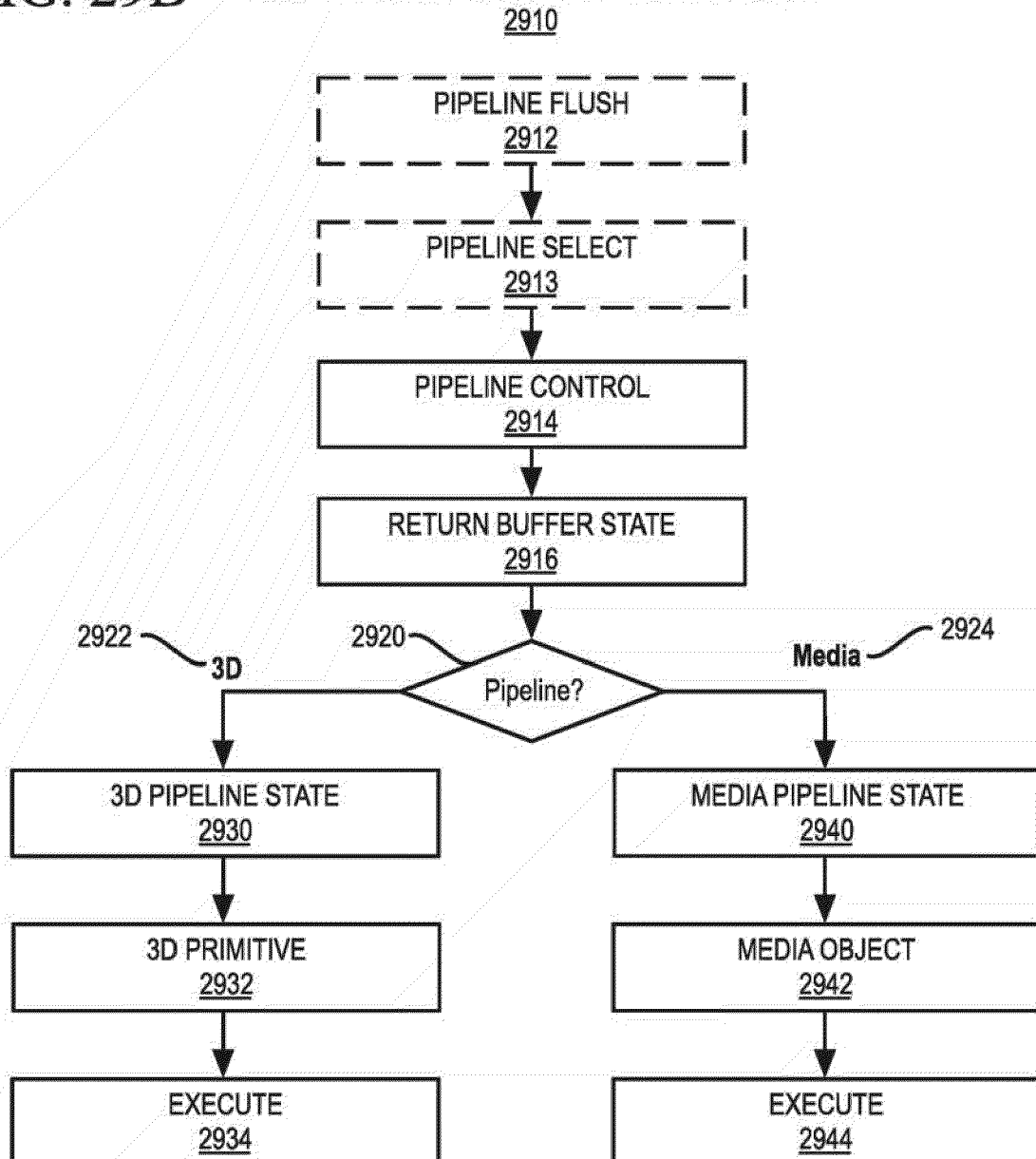
FIG. 29B GRAPHICS PROCESSOR COMMAND SEQUENCE
