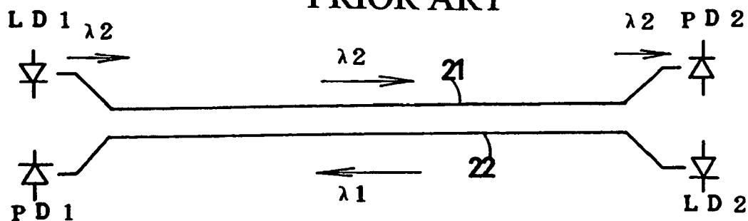
Fig. 3 PRIOR ART
