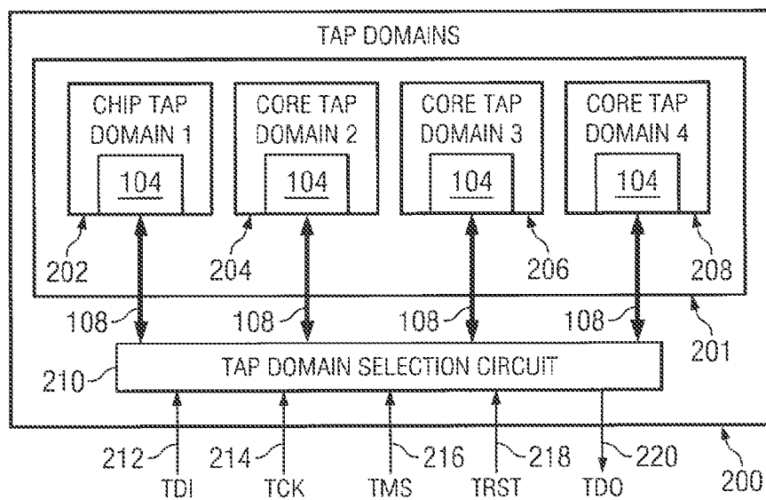
FIG. 2 (PRIOR ART)
