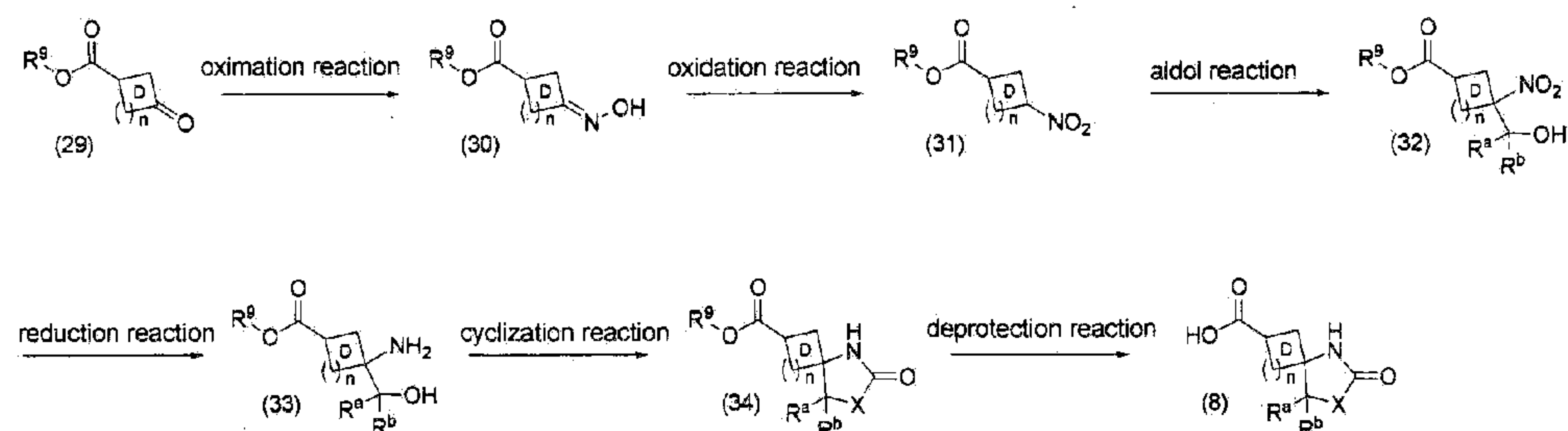
(Scheme 6)
