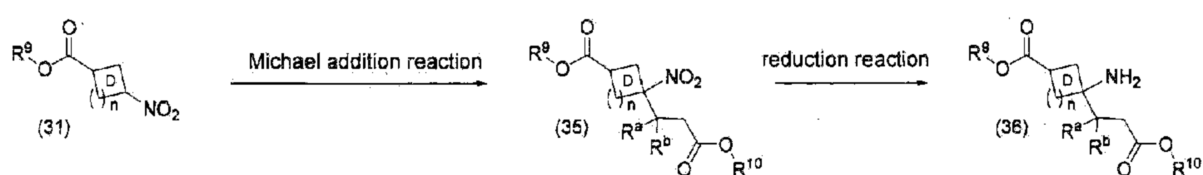
(Scheme 7)
