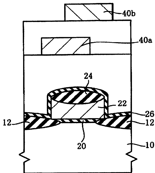
D - D cross section
