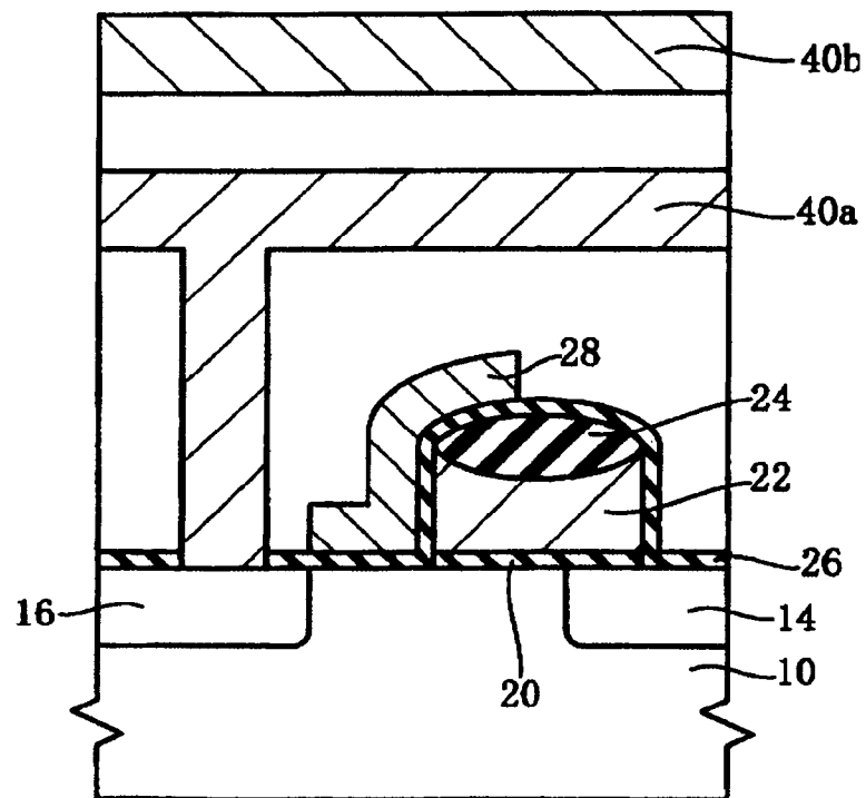
E - E cross section
