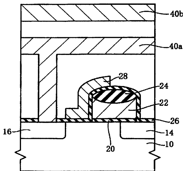
E - E cross section
