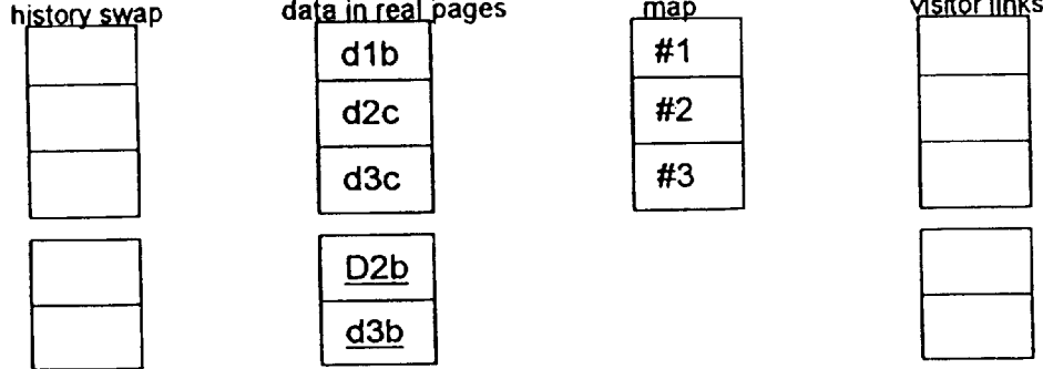
Figure 13I: Swap history pages back in place
