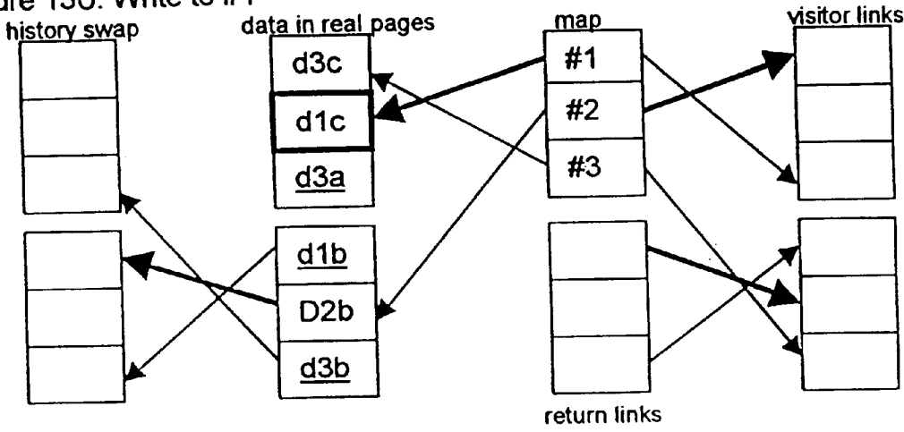
Figure 13U: Write to #1
