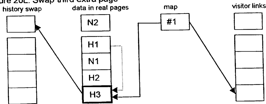
Figure 20L: Swap third extra page
