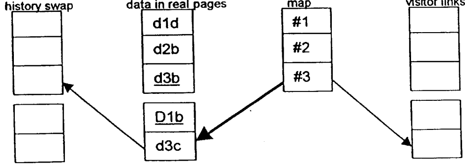
Figure 13L: Swap #2 back in place
