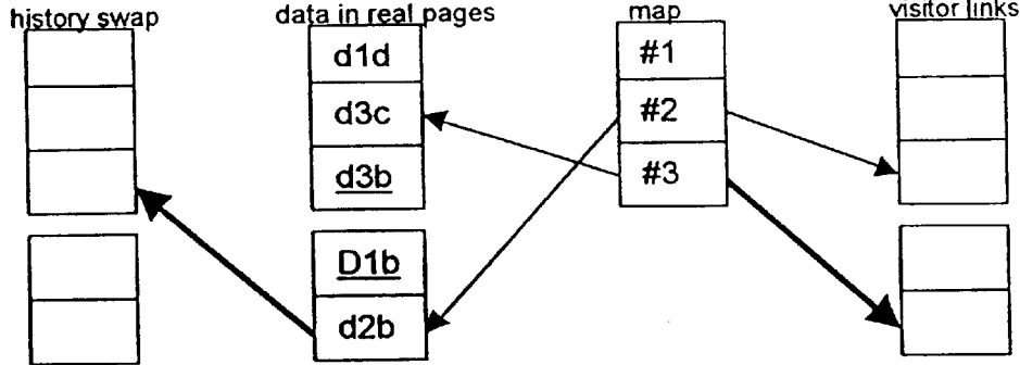
Figure 13K: Swap #1 back in place
