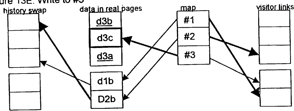
Figure 13E: Write to #3
