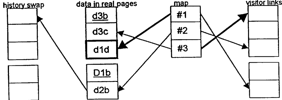
Figure 13J: Write to #1 (following after Figure 13E)
