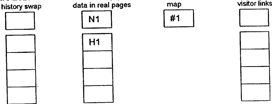
Figure 20B: N1 written and swap performed
