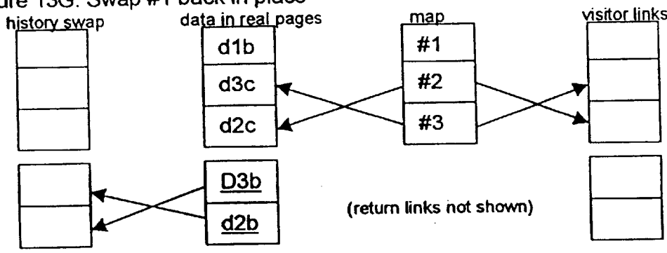
Figure 13G: Swap #1 back in place
