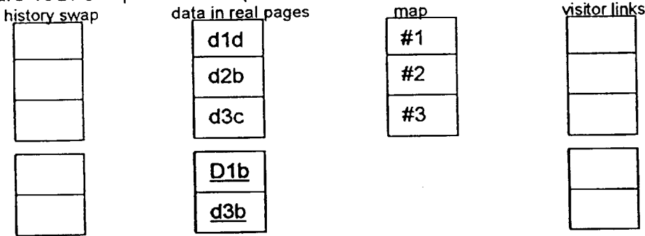
Figure 13O: Swap #3 back in place
