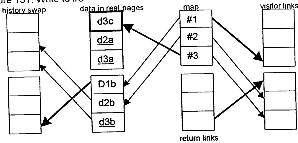
Figure 13T: Write to #3
