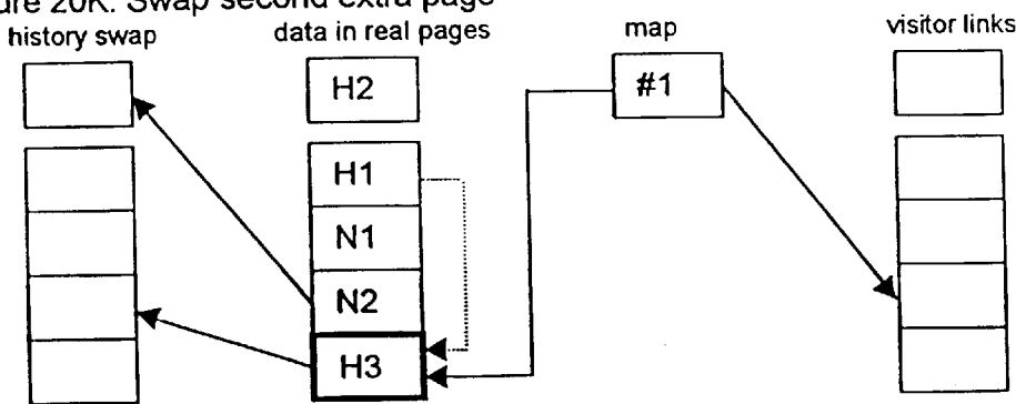
Figure 20K: Swap second extra page
