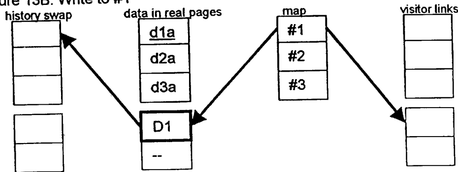
Figure 13B: Write to #1
