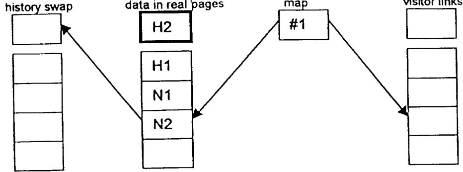
Figure 20E: N2 written
