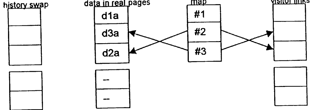
Figure 13Q: Swap #1 back in place
