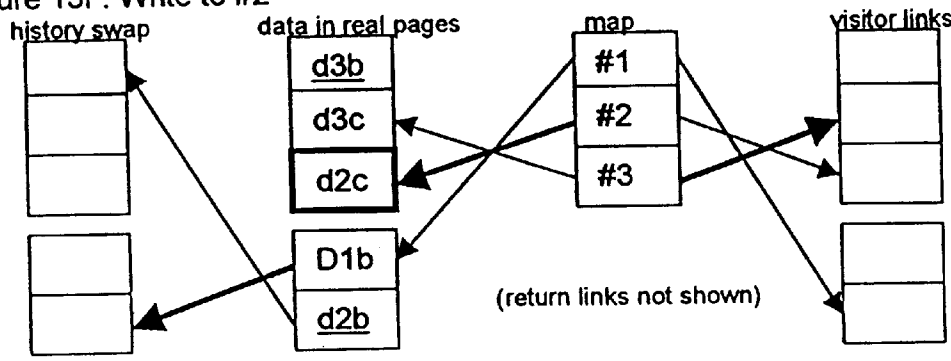
Figure 13F: Write to #2
