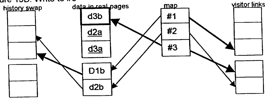
Figure 13D: Write to #3
