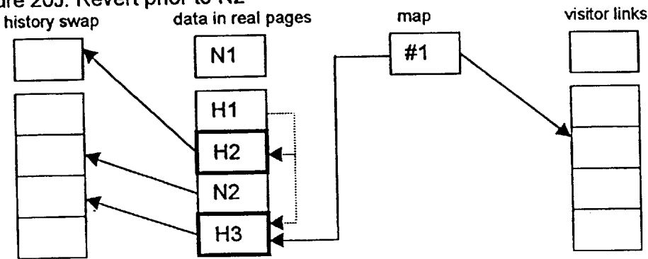
Figure 20J: Revert prior to N2
