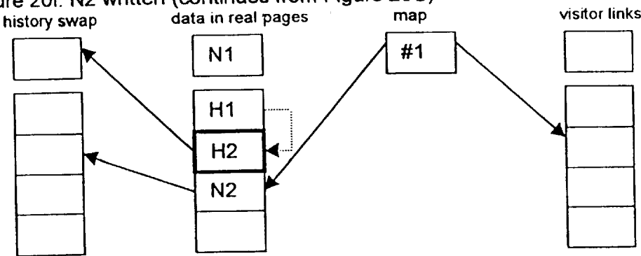
Figure 20I: N2 written (continues from Figure 20C)
