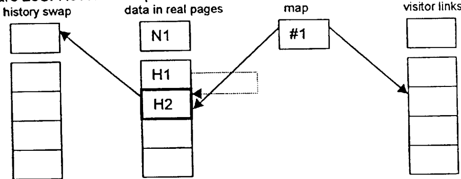
Figure 20C: Revert back prior to N1
