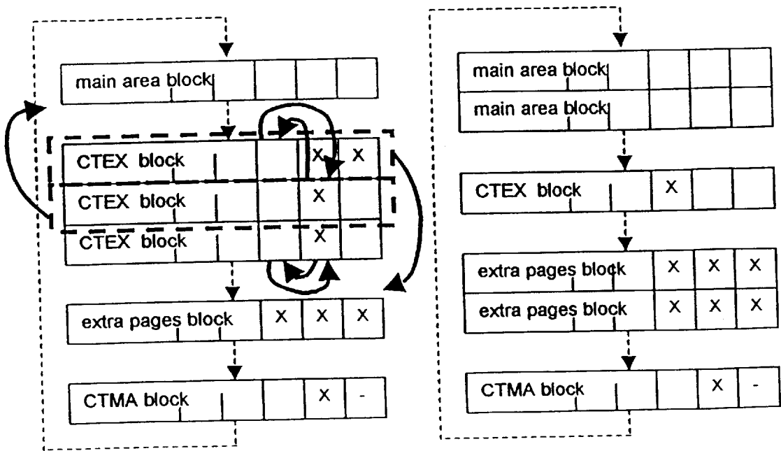
Figure 34 (before and after)
