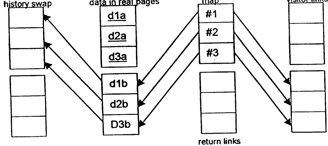
Figure 13S: Write to #1, #2, and #3
