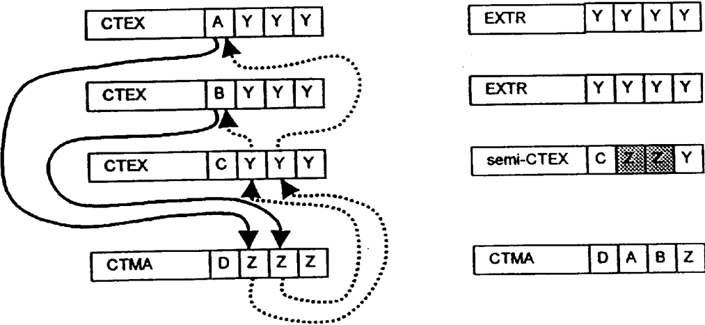
Figure 34P (before and after)
