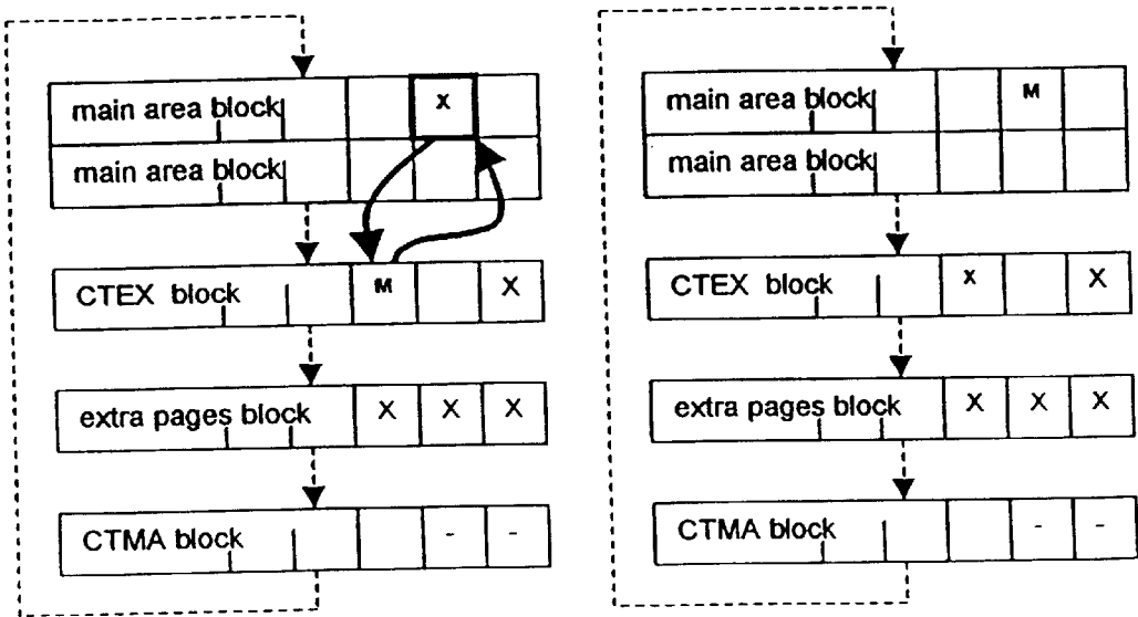
Figure 30 (before and after)
