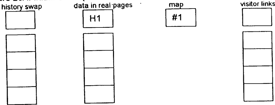
Figure 20A: Initial State (H1 written to location #1)
