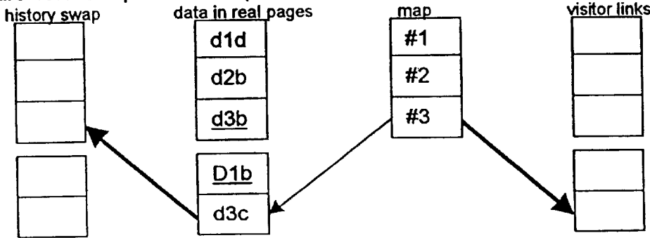
Figure 13N: Swap #1 back in place
