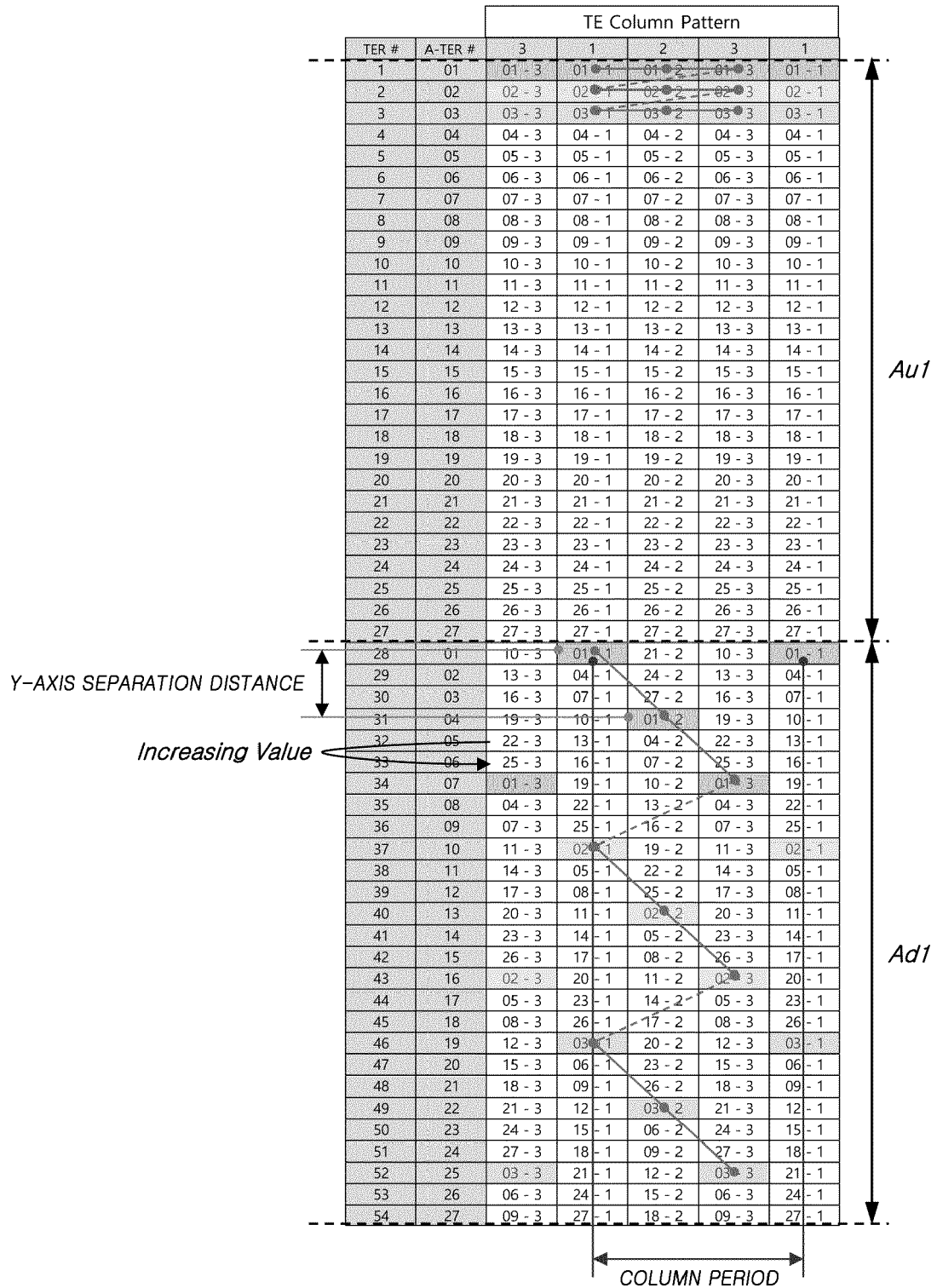
FIG. 11 Touch Allocation Map
