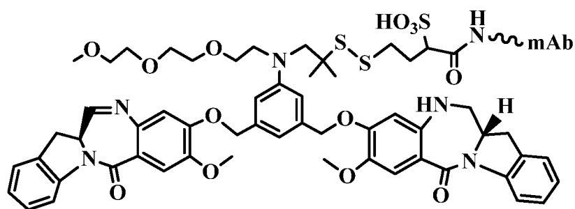
Indolinobenzodiazepine dimer conjugate
