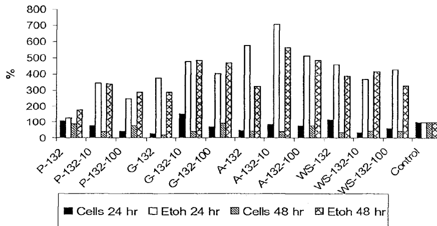
Chart 2C. % Growth and Ethanol Production for P. stipitis
