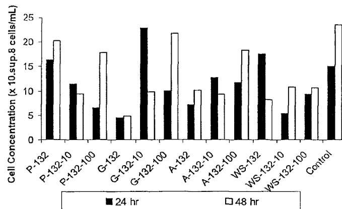
Chart 2A. Cell concentrations for P. stipitis
