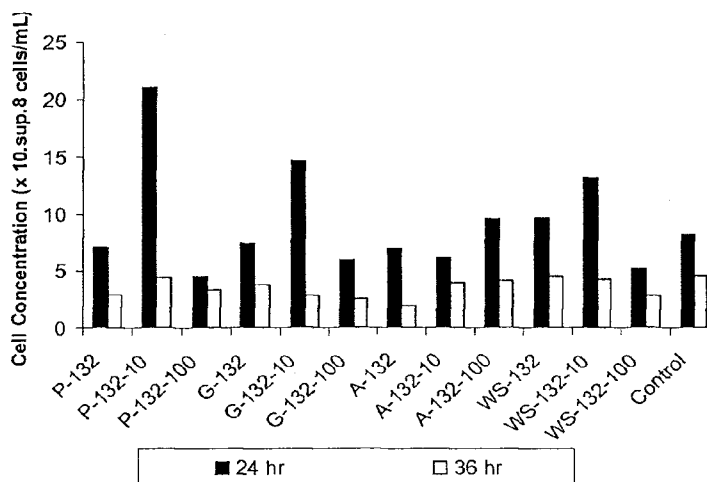
Chart 1A. Cell Concentrations for Z. mobilis
