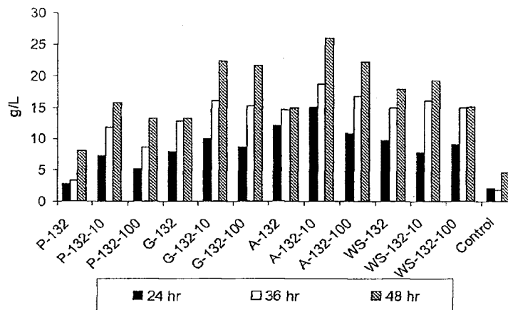
Chart 2B. Ethanol Concentrations for P. stipitis
