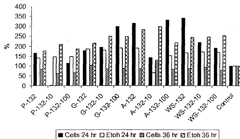
Chart 3C. % Growth and Ethanol Production for S. cerevisiae
