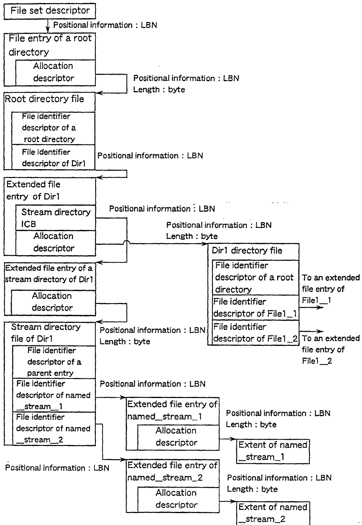
FIG. 46 (PRIOR ART)
