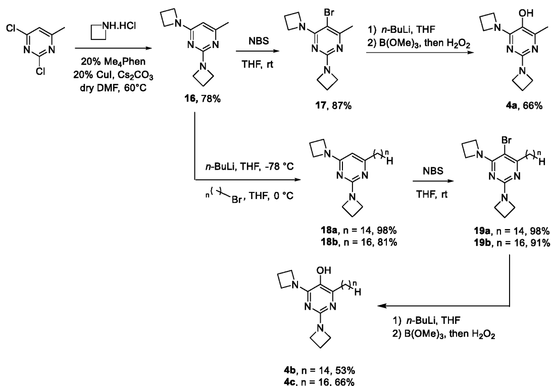
Scheme 3. Synthesis of compounds 4a-c
