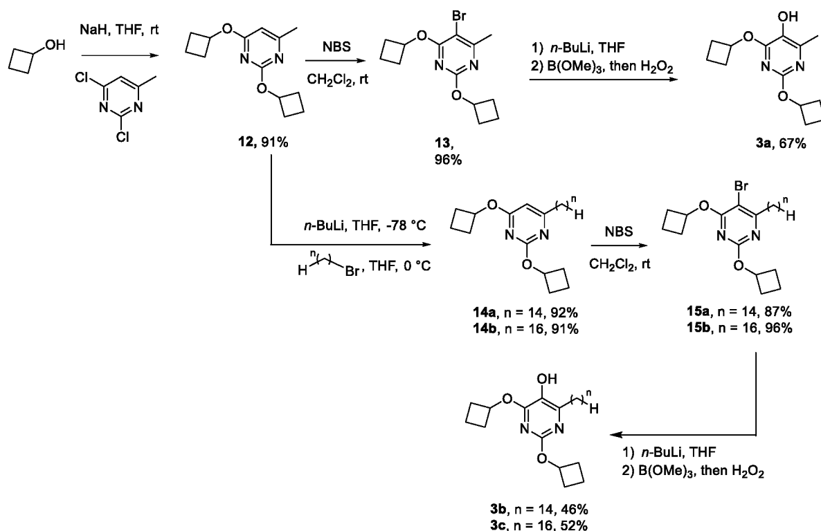
Scheme 2. Synthesis of compounds 3a-c
