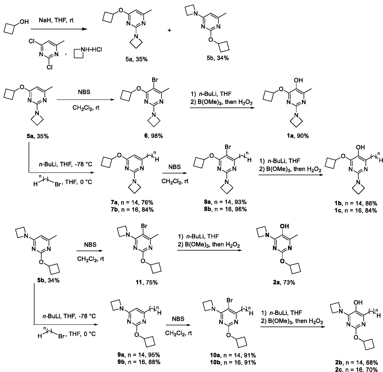
Scheme 1. Synthesis of compounds 1a-c and 2a-c
