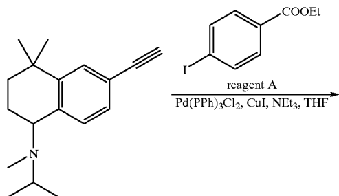
intermediate 29
