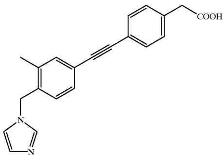
Compound 121
