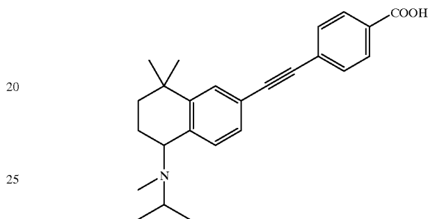
Compound 26
