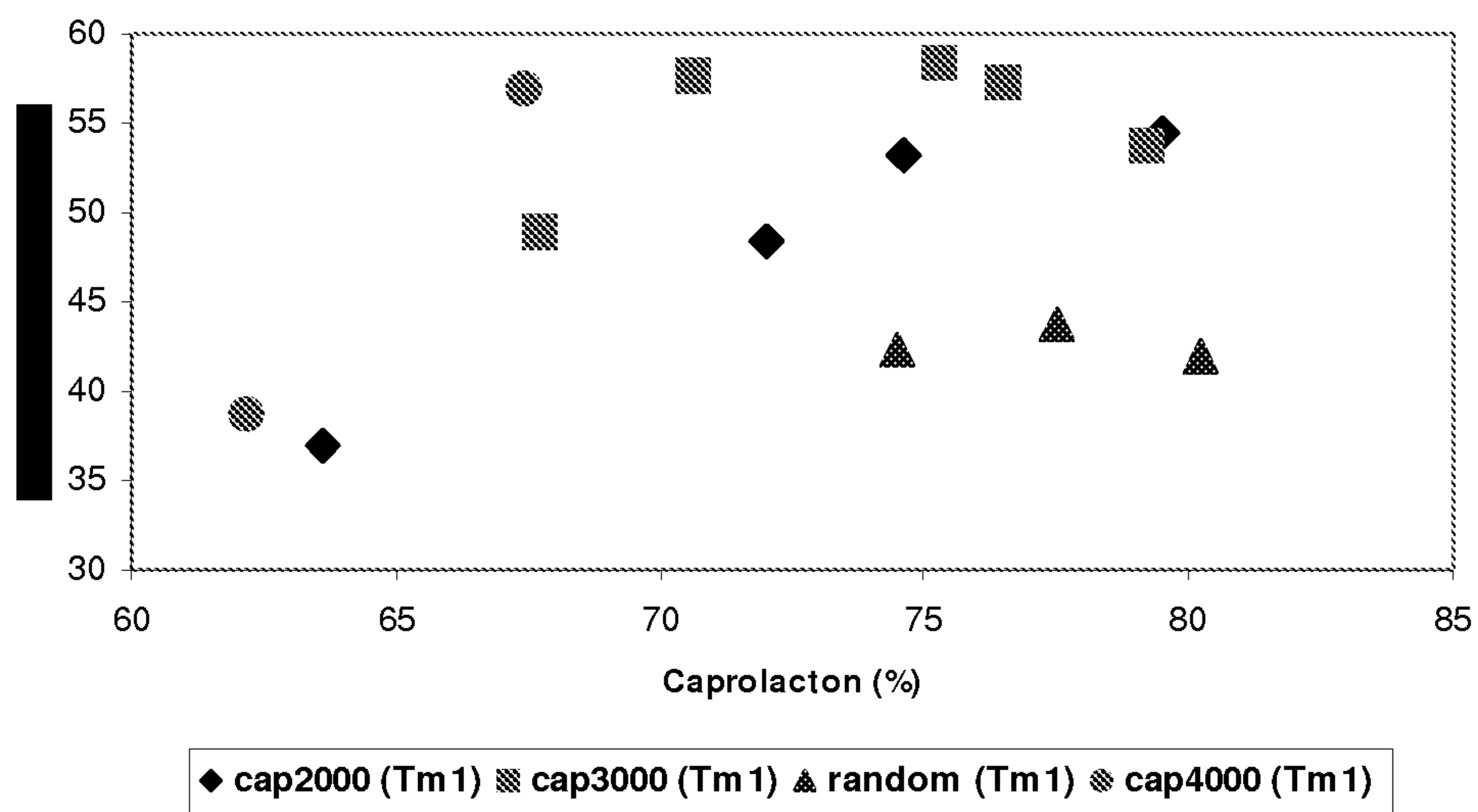
Figure 3: Melting temperature vs caprolactone content
