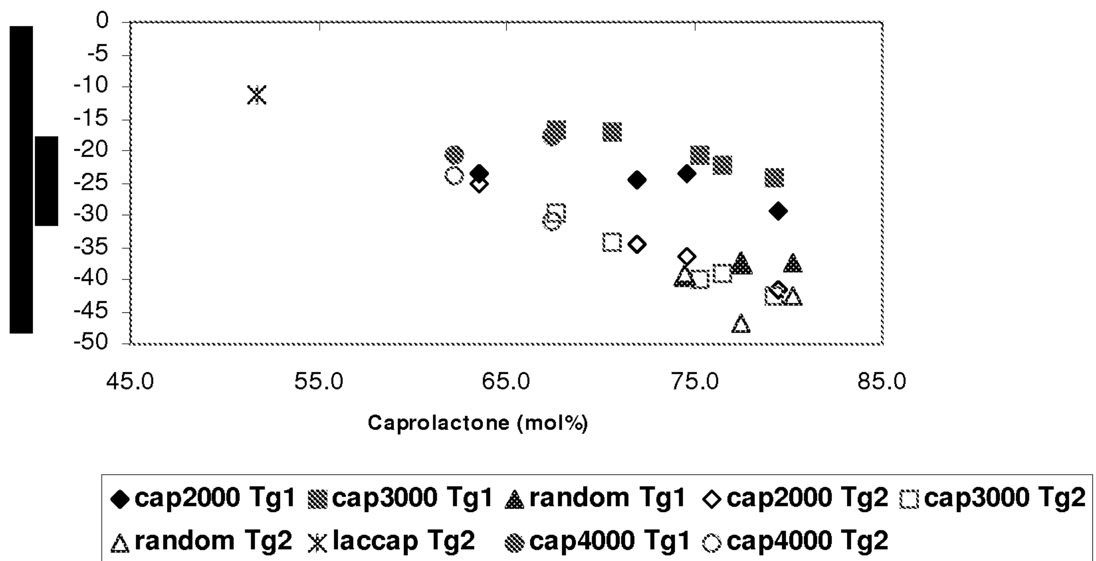
Figure 2: Glass transition temperature vs caprolactone content
