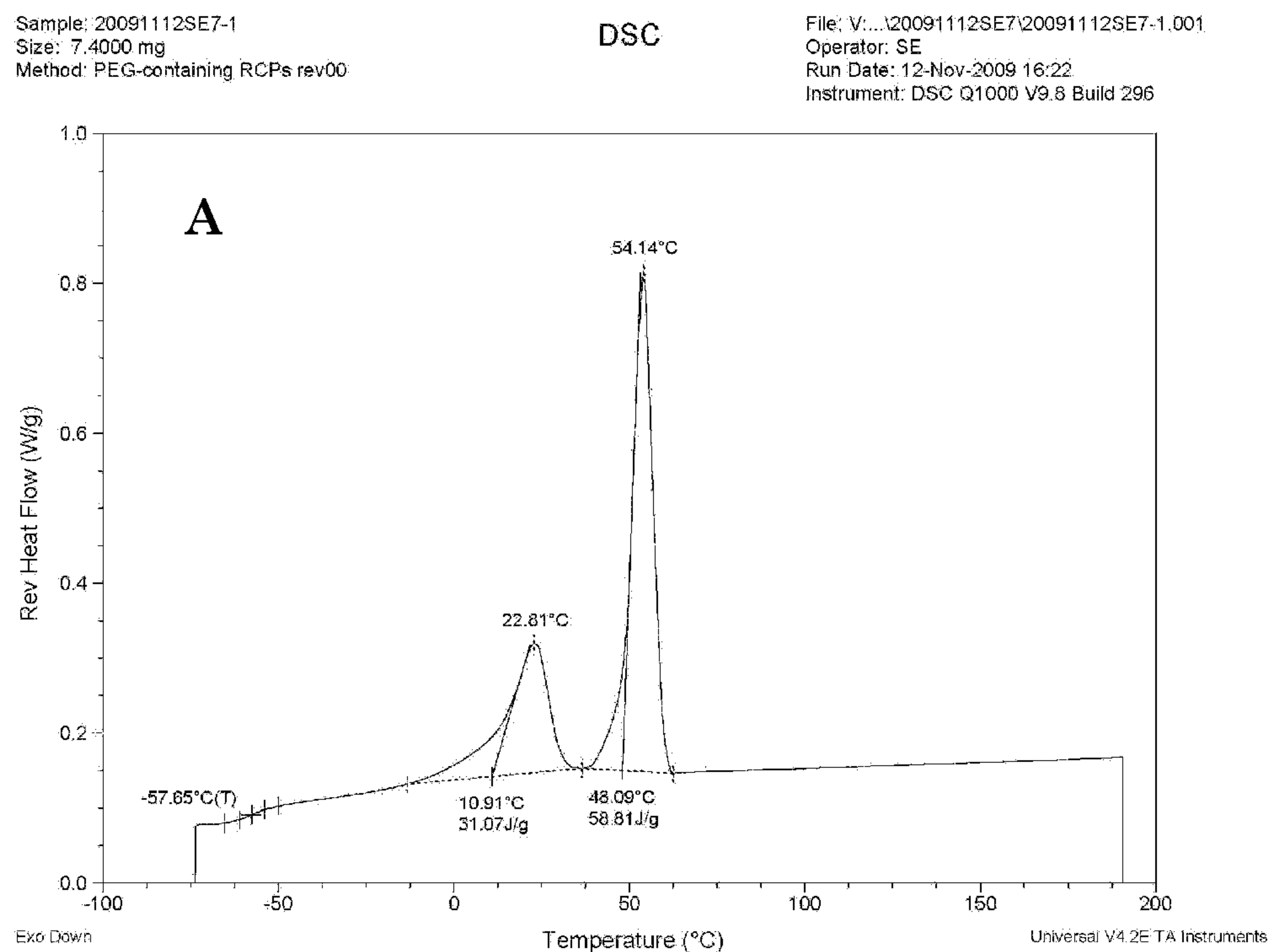
Figure 9 Typical DSC thermograms of 50CLPEG15CL20-b-CL40 (A) and 50LAPEG15LA20-b-CL40 (B). Only reversing heat flow is shown.
