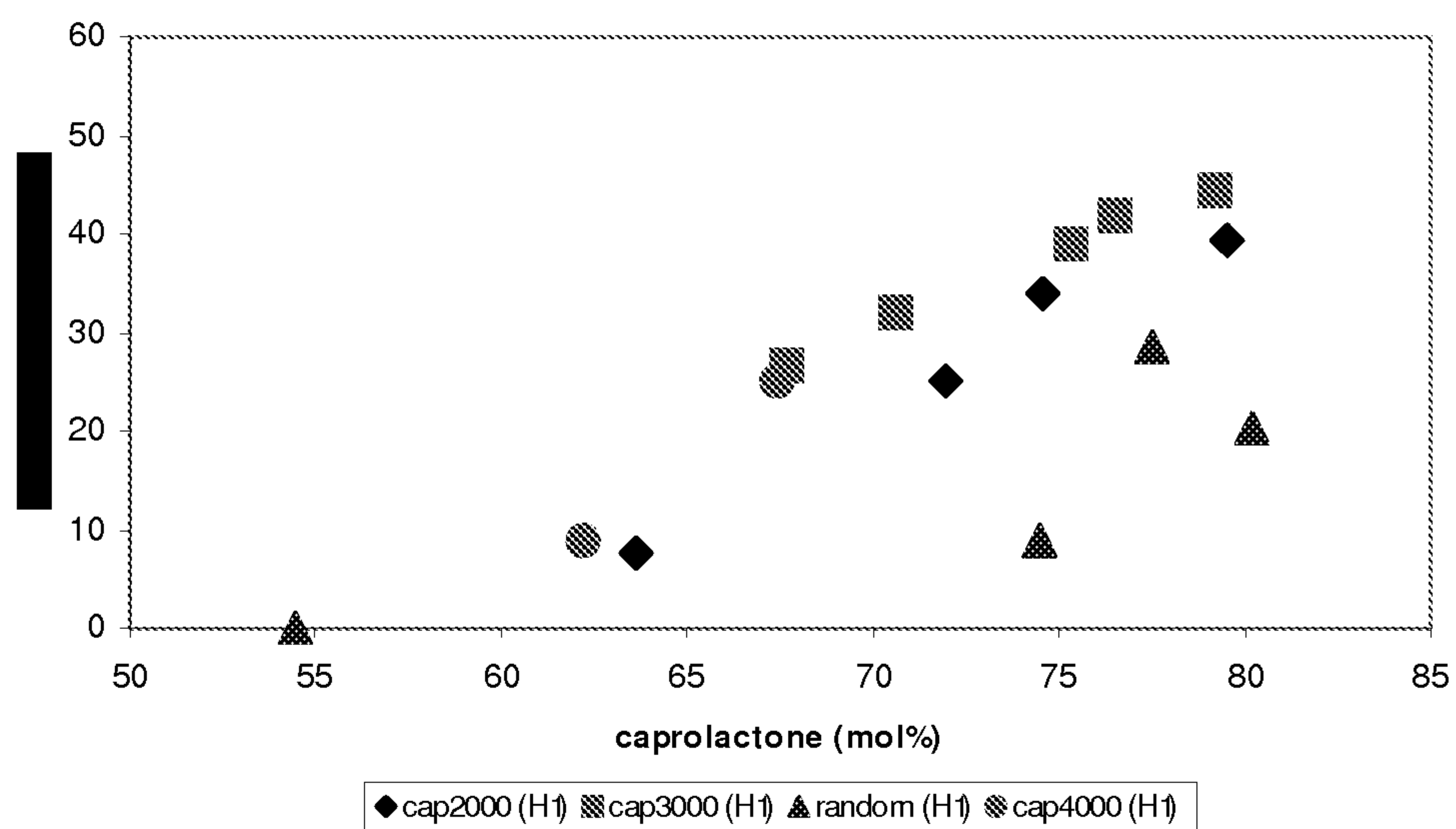
Figure 4: Melting enthalpy vs caprolactone content
