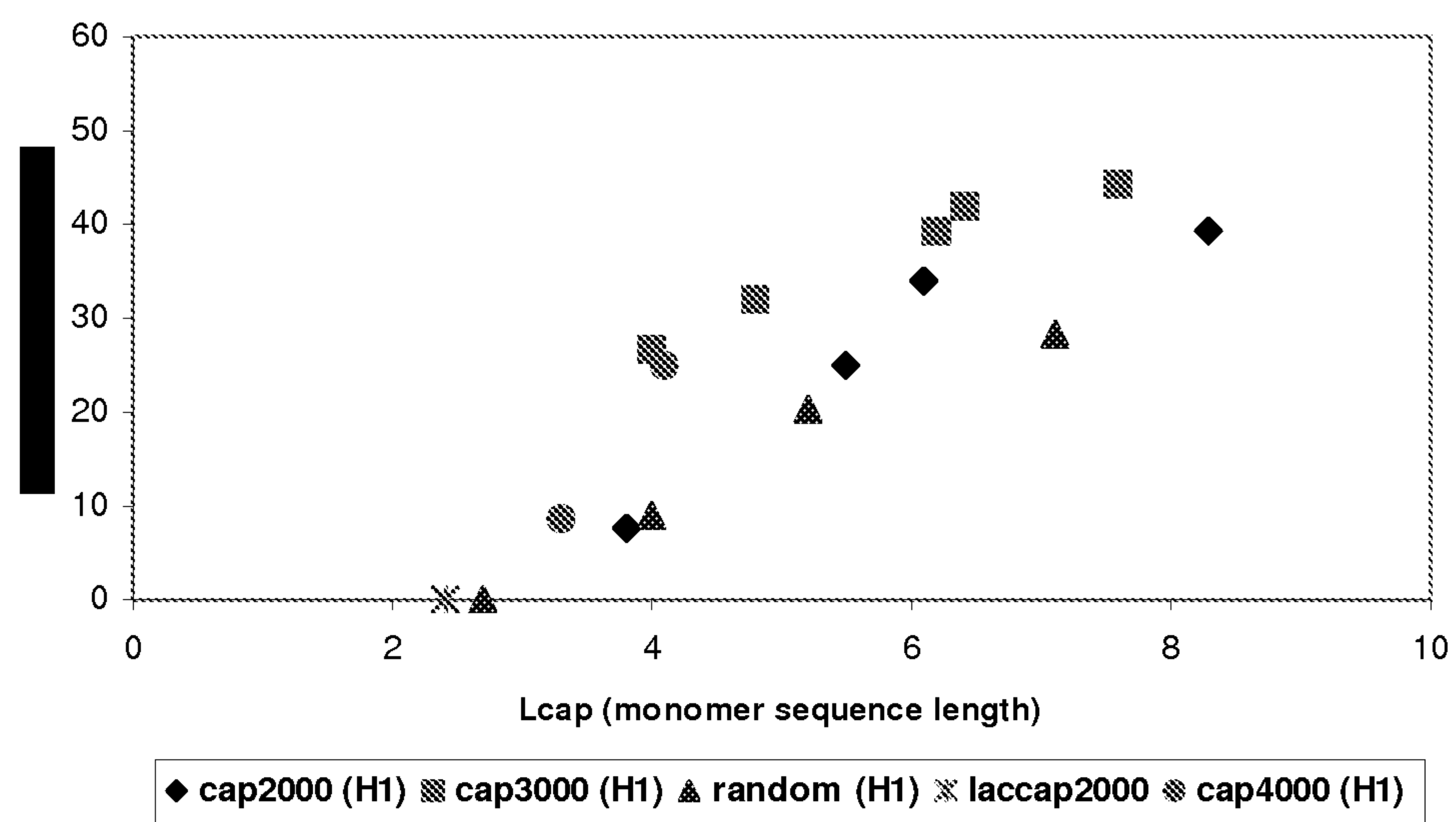
Figure 5: Melting enthalpy vs average caprolactone sequence length
