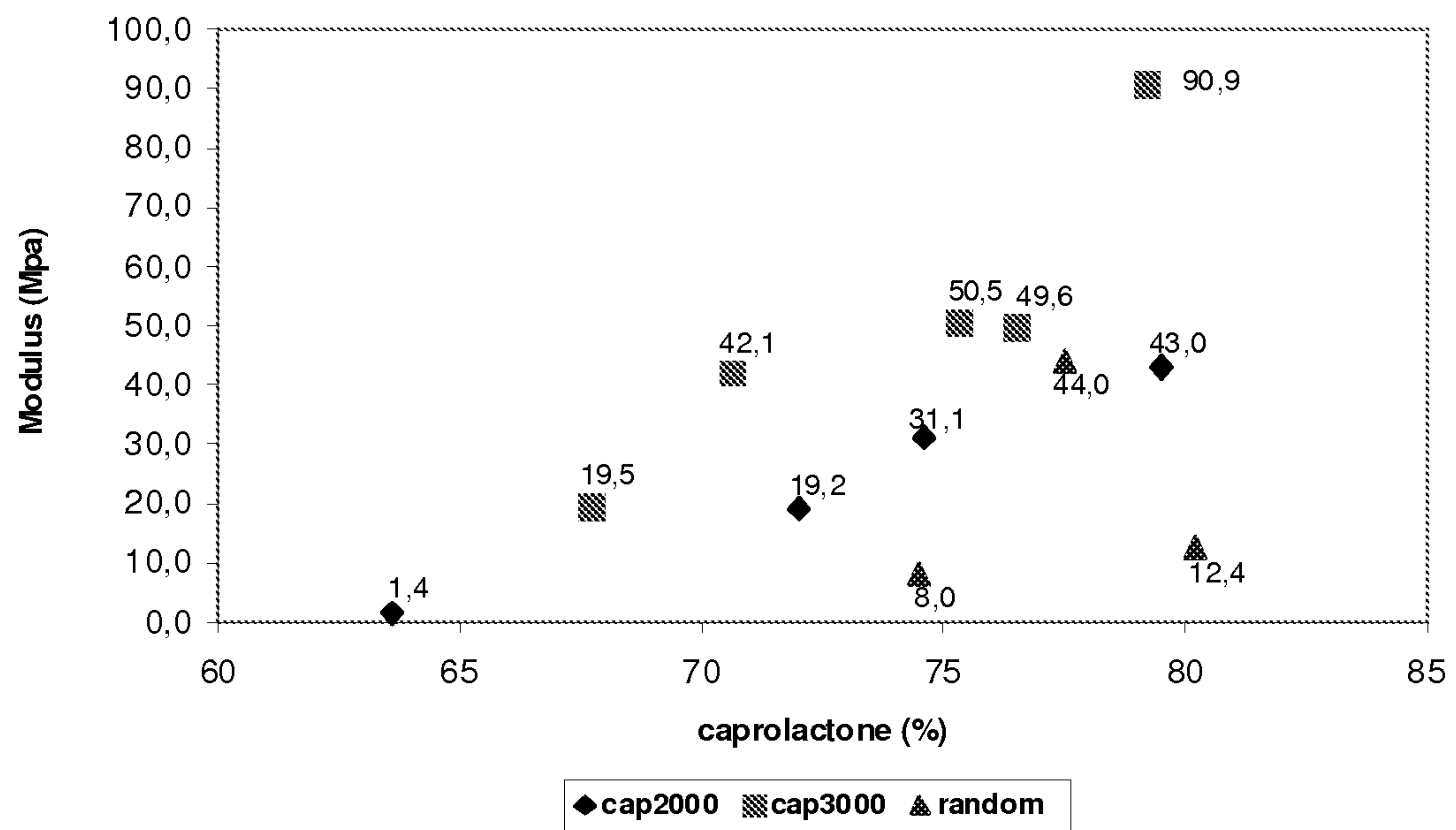
Figure 8: Modulus vs caprolactone content
