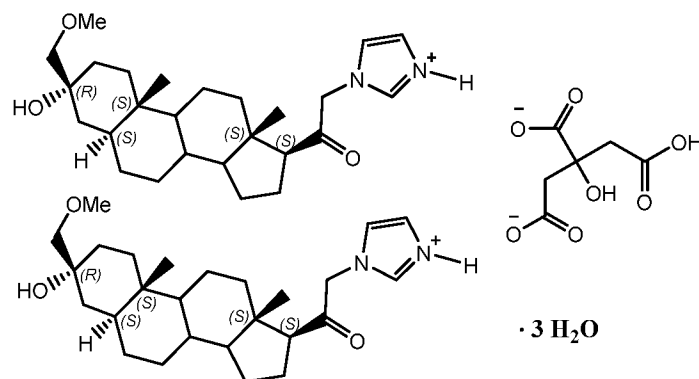
Compound 1 hemi-citrate Sesquihydrate C_{26}H_{40}N_2O_3 \cdot 0.5C_6H_8O_7 \cdot 1.5H_2O 551.71 g/mole
