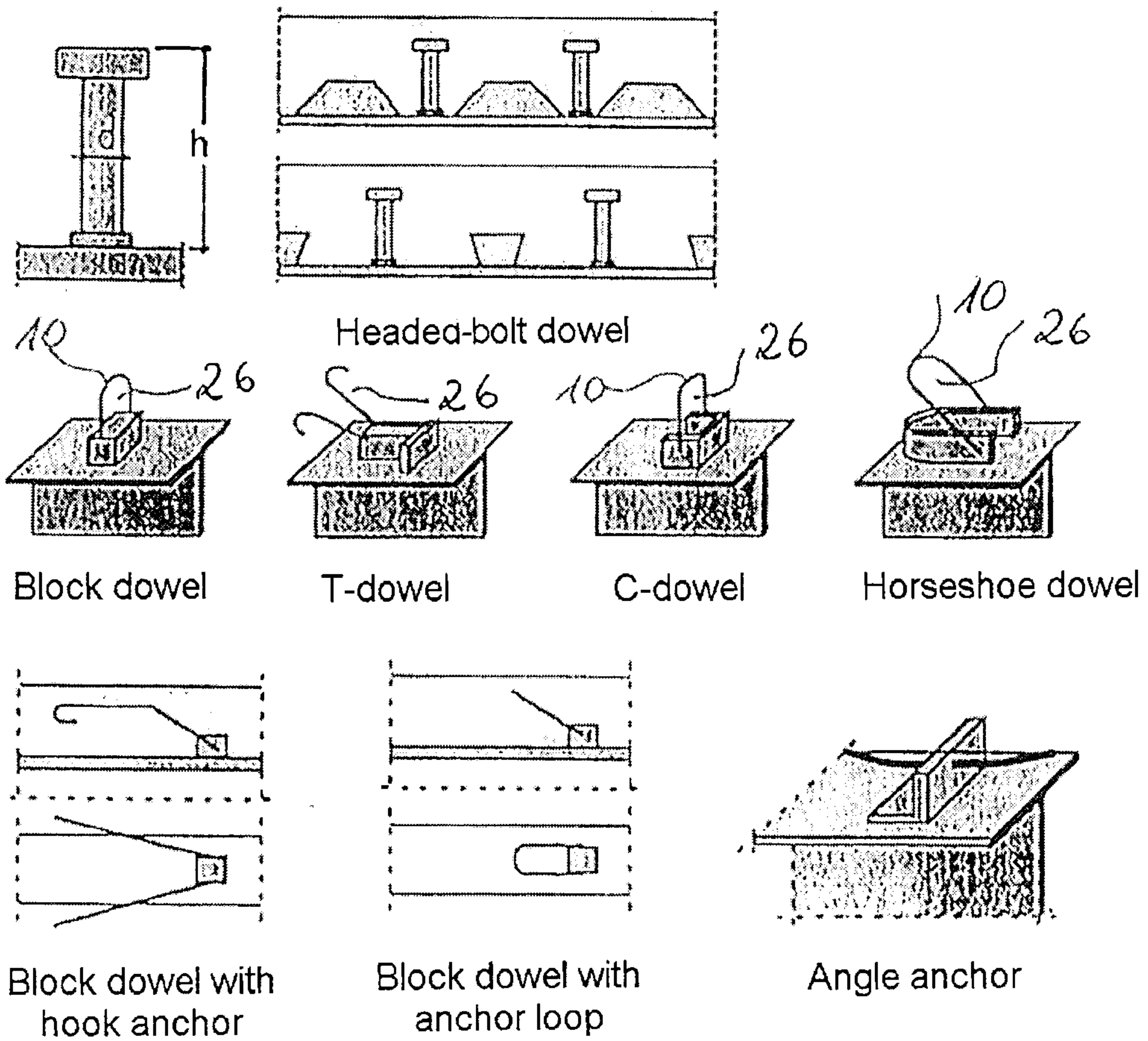
Fig. 3 discontinuous bonding means:
