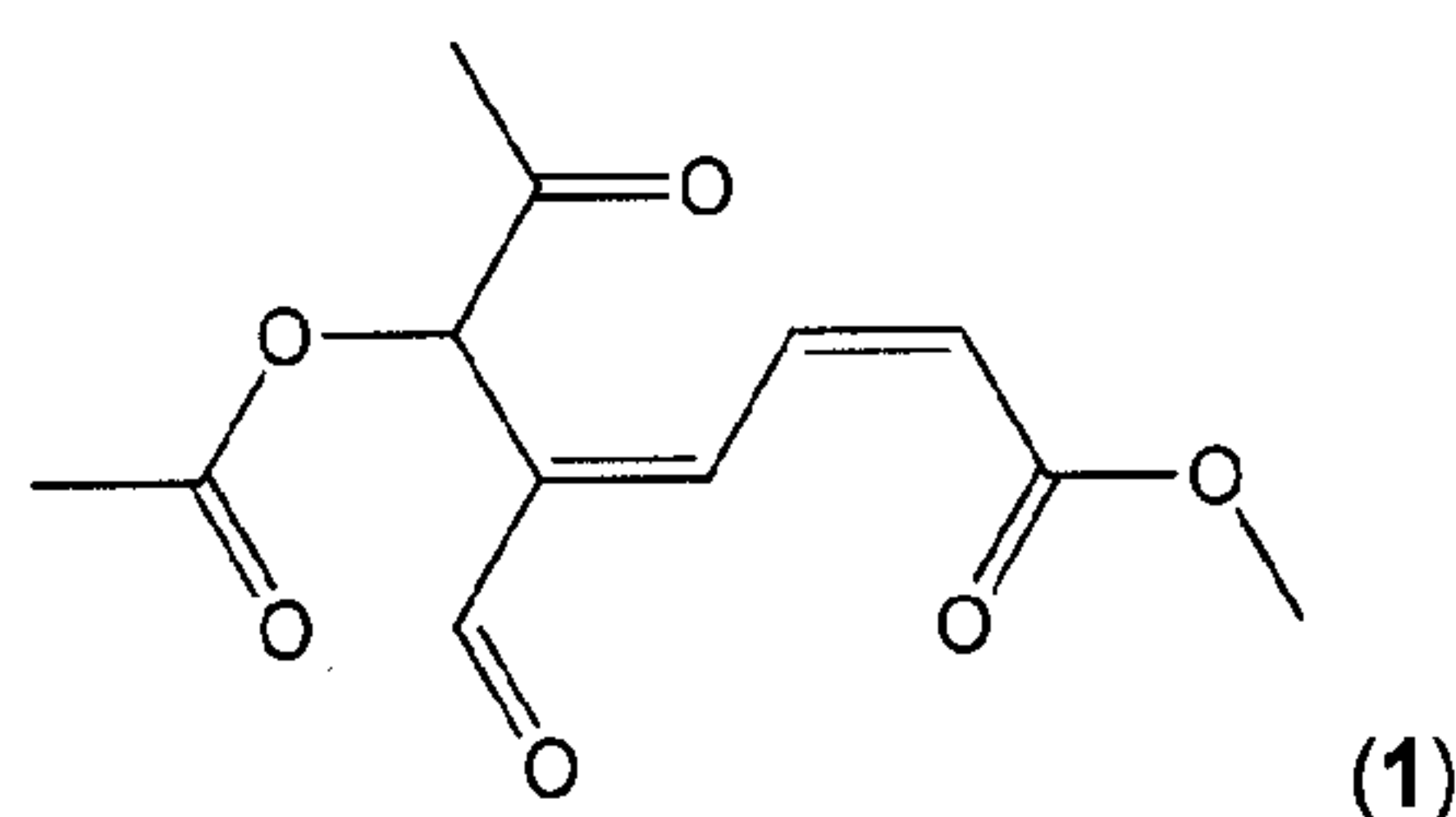
(2Z,4E)-methyl 6-acetoxy-5-formyl-7-oxoocta-2,4-dienoate
