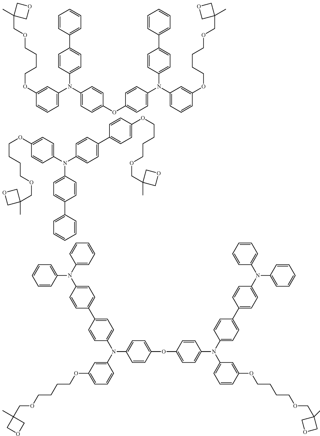
[Chemical Formula 1]
