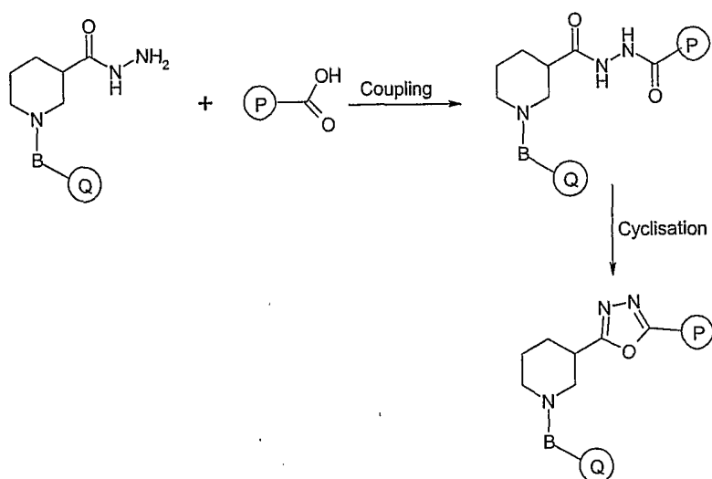
Scheme 21
