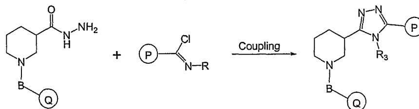
Scheme 19
