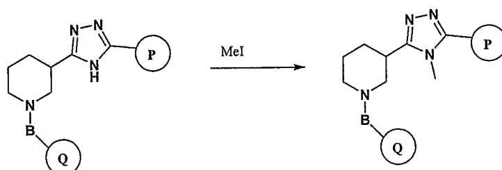
Scheme 17
