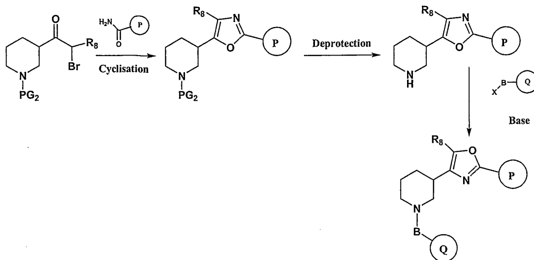
Scheme 23
