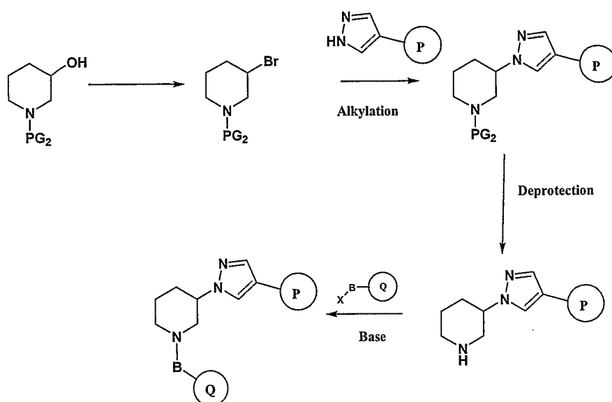
Scheme 30
