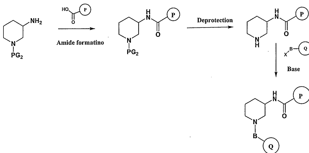
Scheme 34
