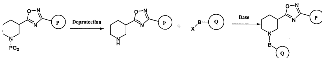
Scheme 9
