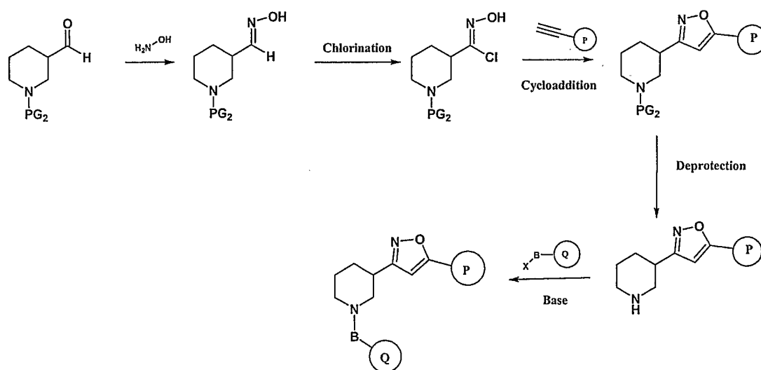
Scheme 25
