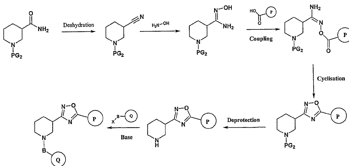
Scheme 16
