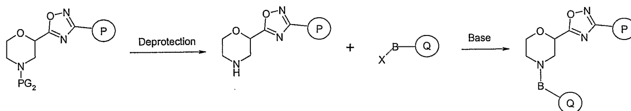
Scheme 12
