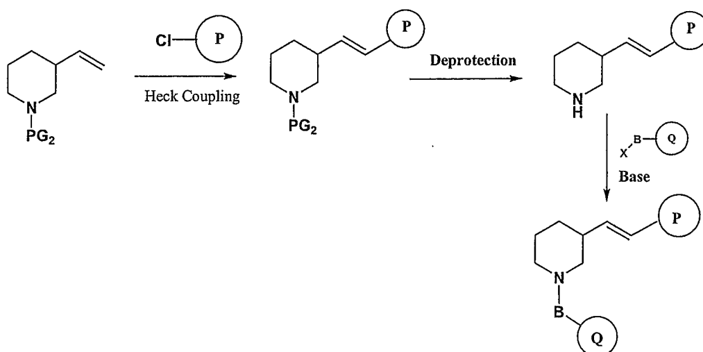
Scheme 32
