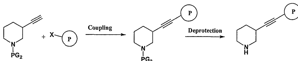
Scheme 5
