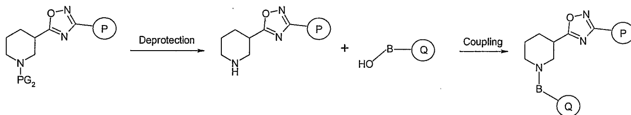
Scheme 10
