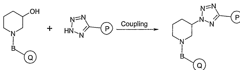
Scheme 29
