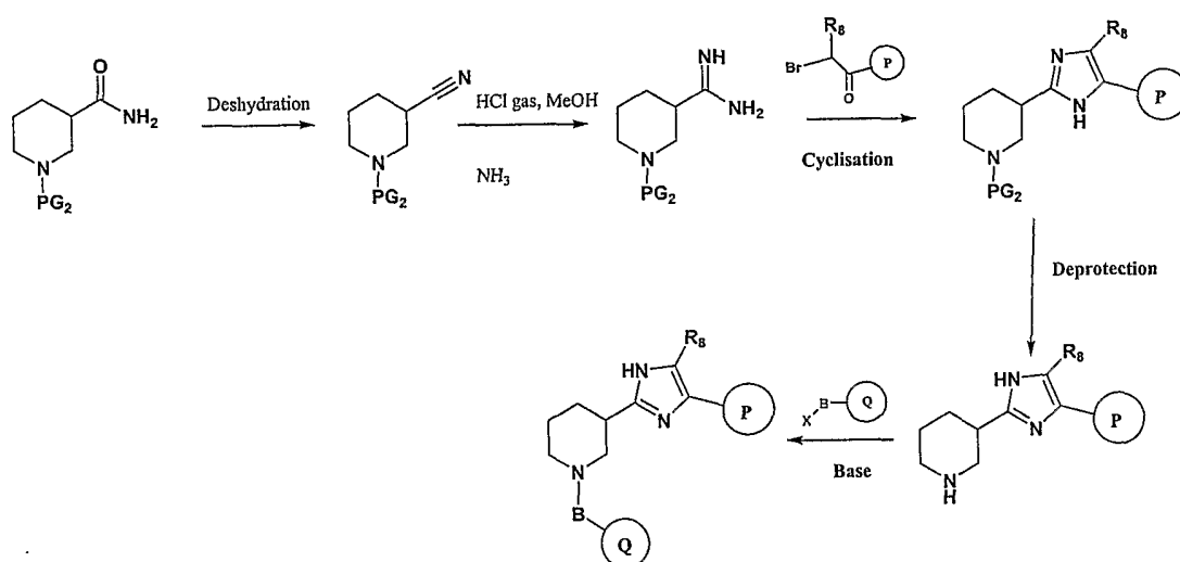
Scheme 26
