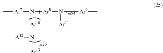
[Chemical Formula 41]
