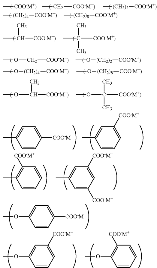
[Chemical Formula 10]
