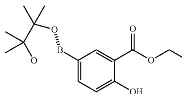
[Chemical Formula 81]
