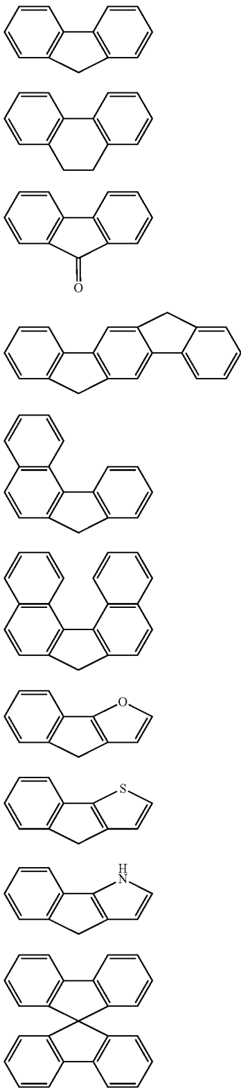
[Chemical Formula 40]
