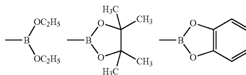
[Chemical Formula 73]
