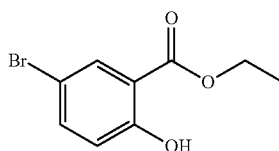
[Chemical Formula 80]
