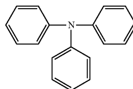
[Chemical Formula 42]
