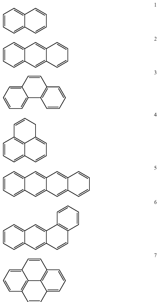
[Chemical Formula 8]
