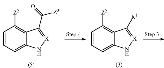
Reaction Scheme 2
