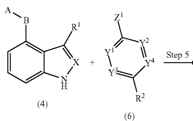
Reaction Scheme 3
