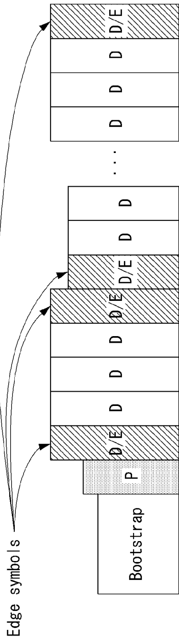
(b) Two edge symbols per sub-frame for a mixed FFT frame
