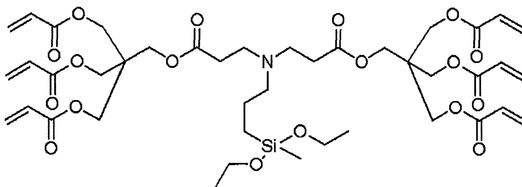
Polymerizable Compound 2
