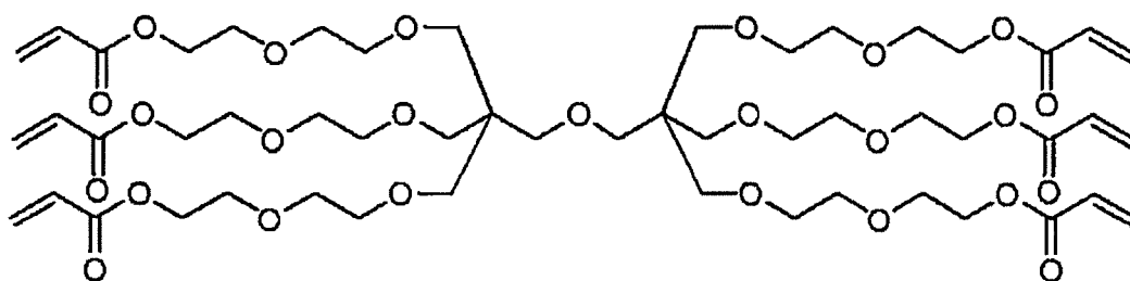
Polymerizable Compound 3
