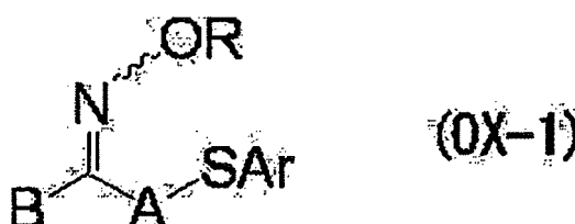
[Chem. 2]
