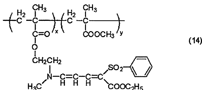
[Chem. 21]
