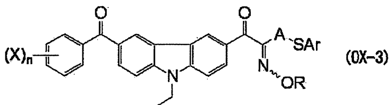
[Chem. 7]
