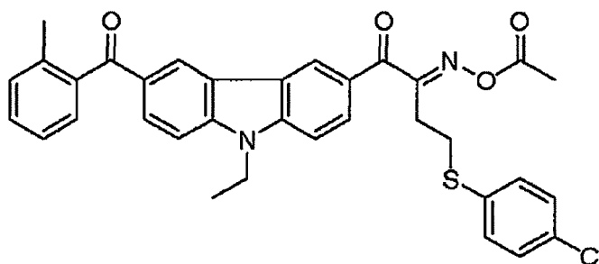
[Chem. 31]
