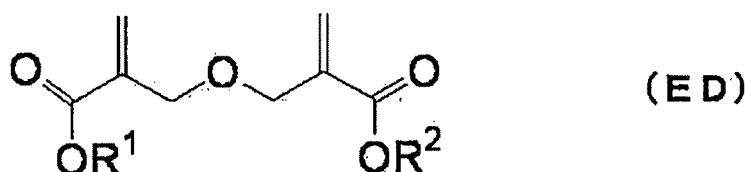
[Chem. 22]
